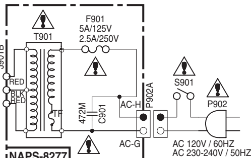
U03 POWER TRANSFORMER PC BOARD
