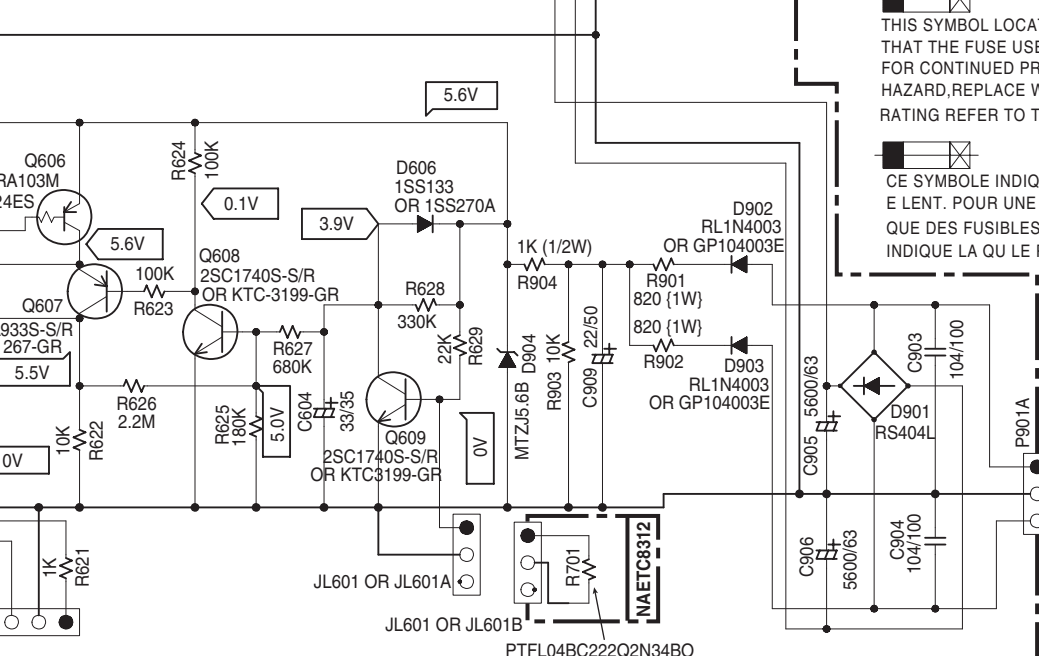
U04 THERMAL SENSOR PC BOARD
