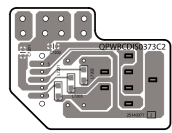
U0044 BAETC-0377 (HP JACK PC BOARD) B-side(Soldering side)
