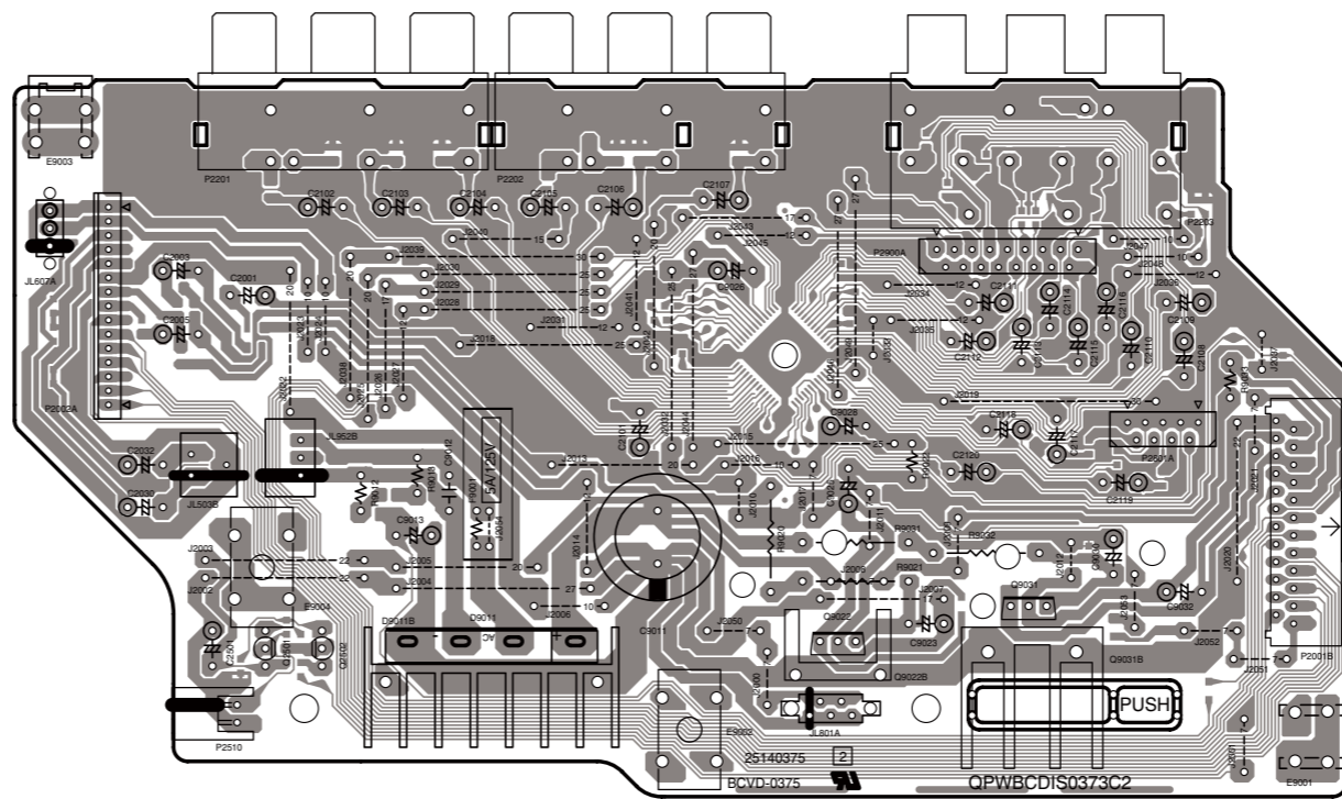
BADIS-0375 (VIDEO PC BOARD) A-side(Component side)
