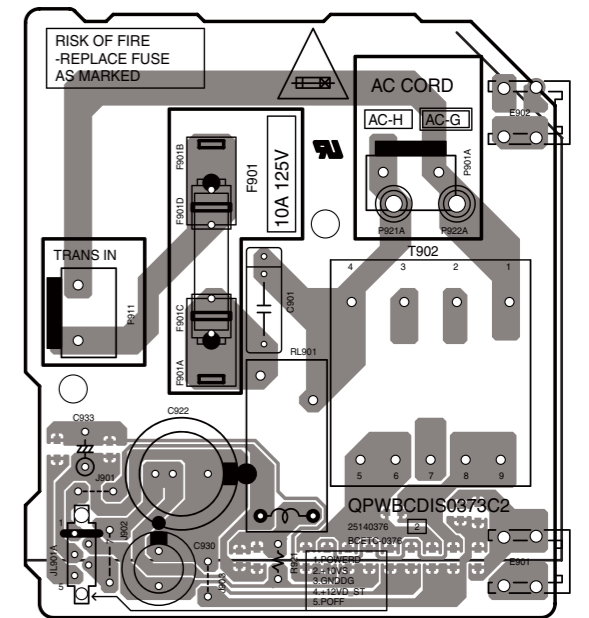
BAETC-0376 (POW SUPPLY PC BOARD) A-side(Component side)
