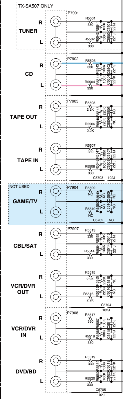
U0011 TRANS 2ND TERMINAL PC BOARD
