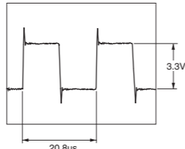
20.8us Front L/R audio data
