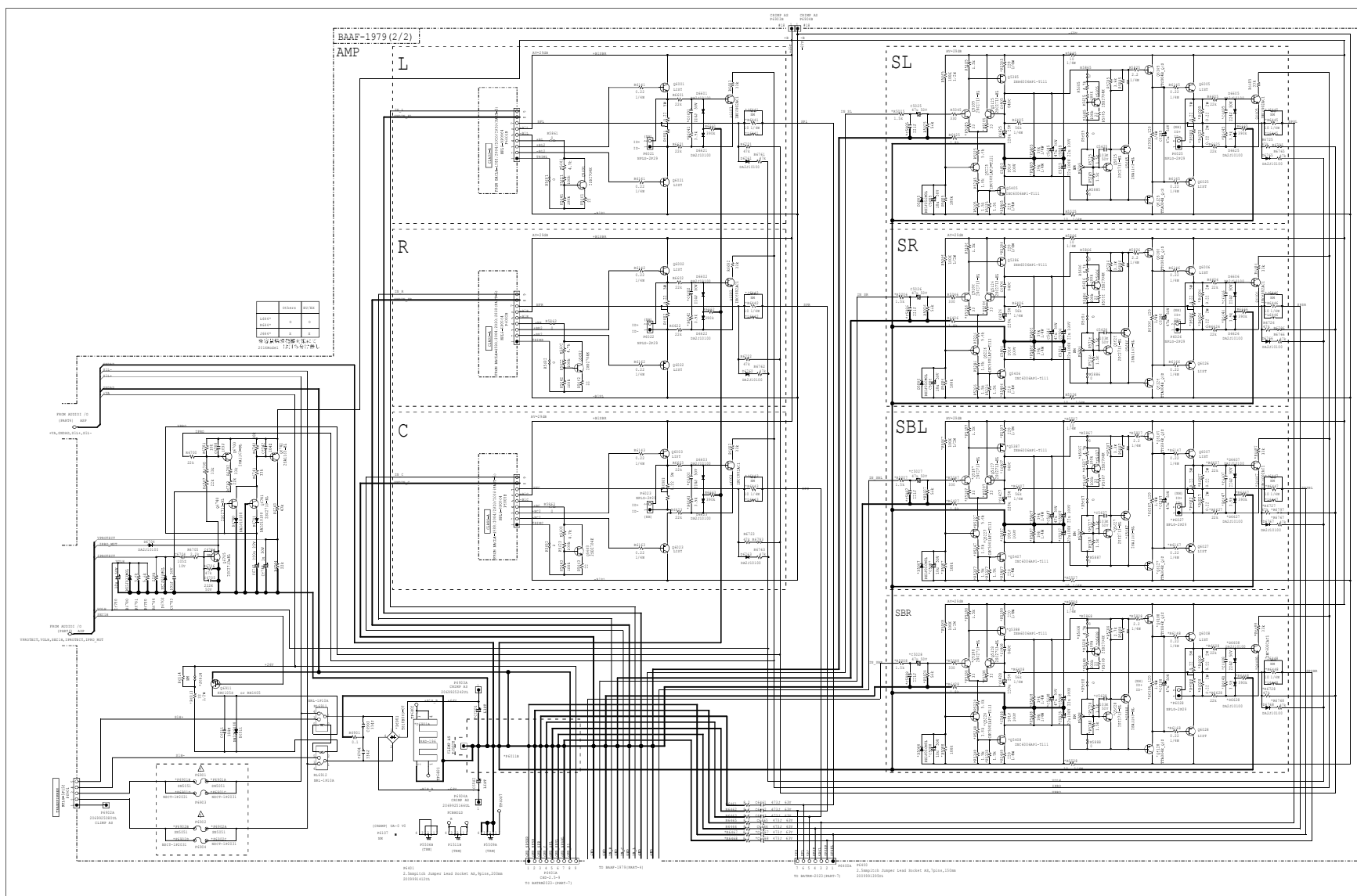
MODELNO.TX-NR555/656/757,TX-RZ610/710/810,HT-R695,DRX-2/3/4/5 SCHEMATIC DIAGRAM (PART-4) AMP SECTION
