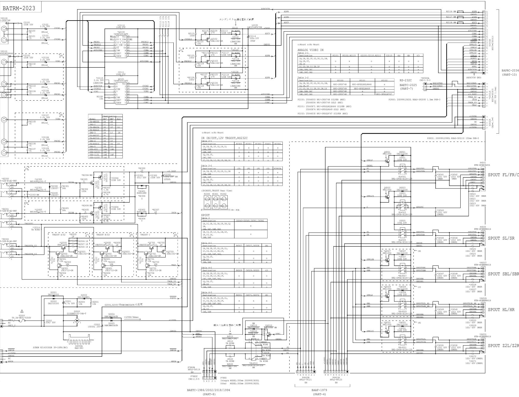
MODEL NO.TX-NR555/656/757,TX-RZ610/710/810,HT-R695,DRX-2/3/4/5 SCHEMATIC DIAGRAM(PART-7) VIDEO, SPOUT,IR/12VTRG SECTION
