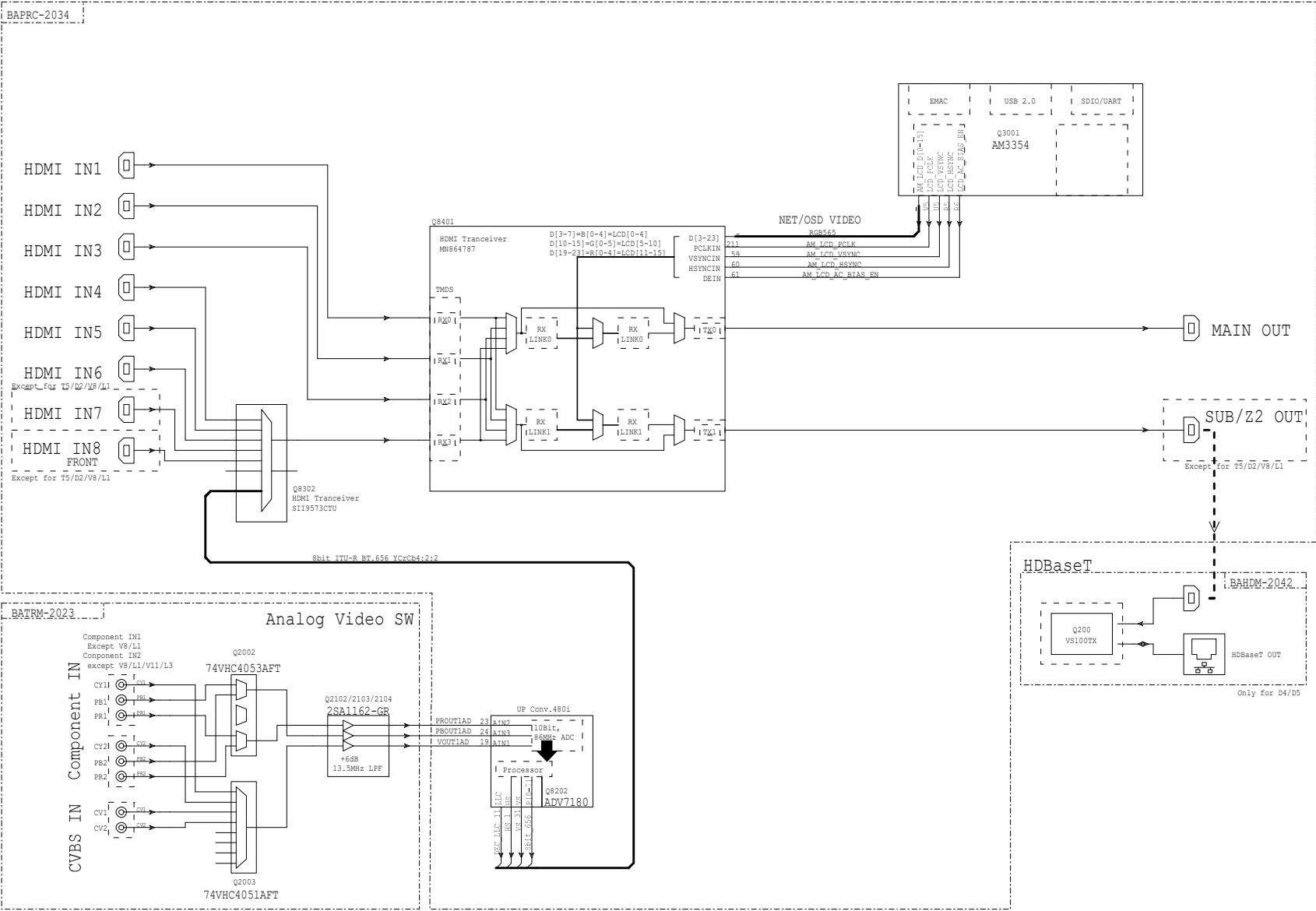
SCHEMATIC DIAGRAM (PART-2) BLOCK DIAGRAM(Video)
