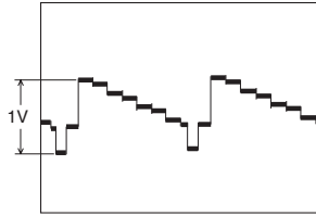
Component PB waveform
