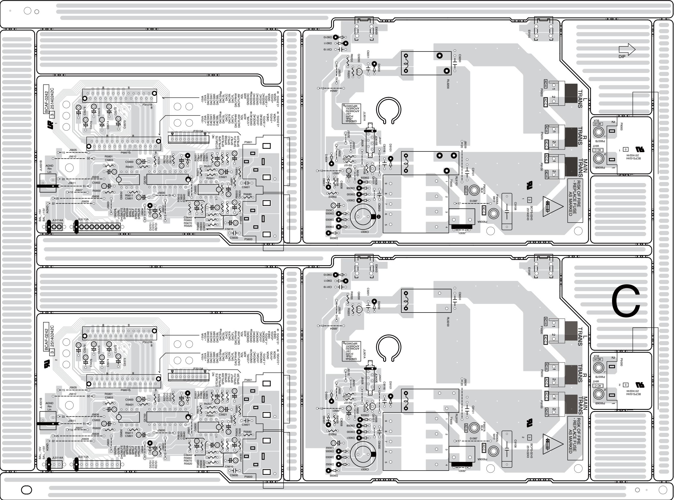
Component side view from solderin side
