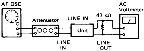
Connection diagram
