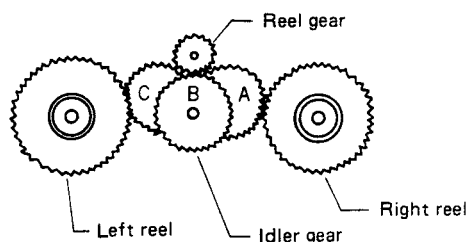
Figure 1: Frontal View of the Assist/Reel Drive Train
