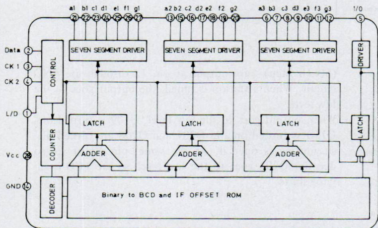
(fig. 8) TD6301AP block diagram
