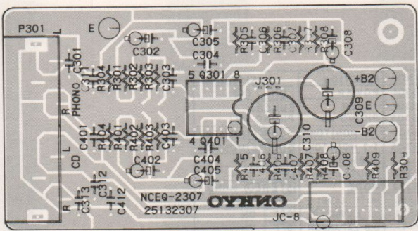
EQUALIZER AMPLIFIER PC BOARD
