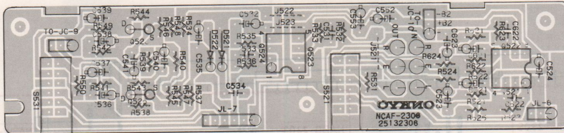
DYNAMIC BASS AND STEREO IMAGE CIRCUIT PC BOARD
