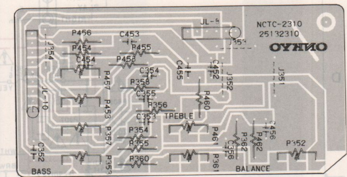
TONE CONTROL CIRCUIT PC BOARD (NATC-2310)
