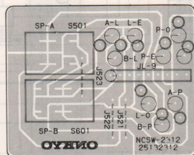
SPEAKER SWITCH PC BOARD
