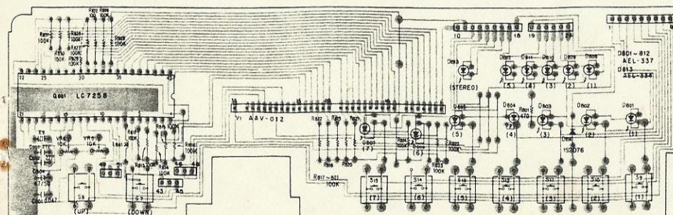
FL assembly (GWX-653)
