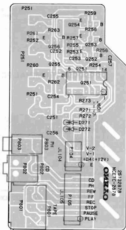
REMOTE CONTROL TERMINAL PC BOARD
