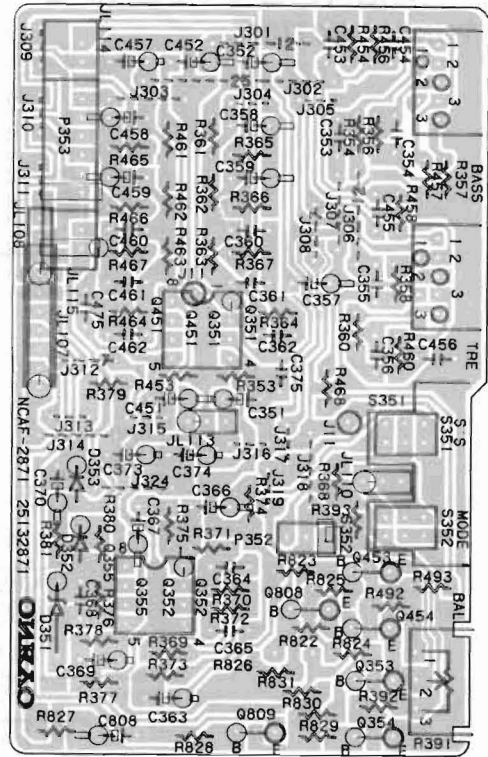
PREAMPLIFIER PC BOARD
