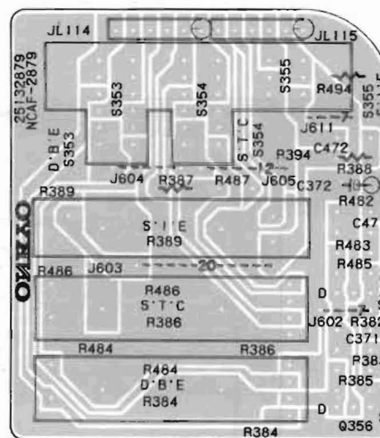
SWITCH PC BOARD
