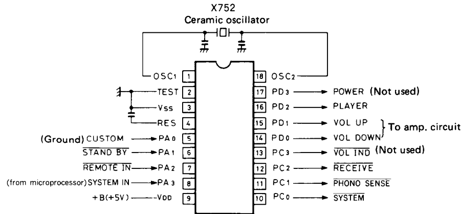
Connection diagram
