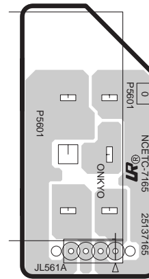
U6 COMPONENT SIDE FRONT SPEAKER TERMINAL PC BOARD
