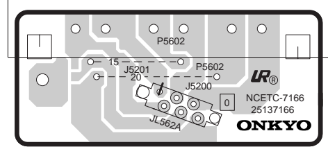
U7 COMPONENT SIDE SURROUND SPEAKER TERMINAL PC BOARD
