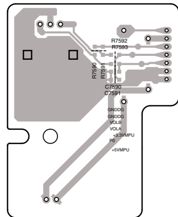
U0054 VOLUME PC BOARD (BAETC-0139) Soldering side view from component side
