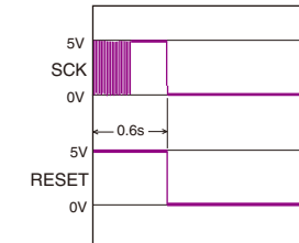
SCK/RESET waveform (WF63) SD-14:F4,H4 SD-16:F4,H4
