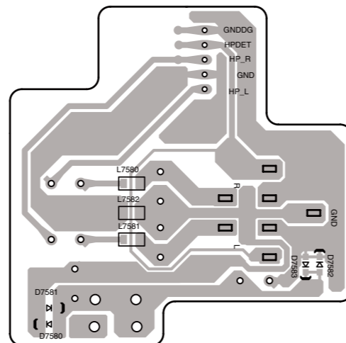
U0052 HEADPHONE JACK PC BOARD (BAETC-0137) Soldering side view from component side
