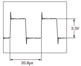
(WF06) DATA3_PLD (SD-12:I7)
