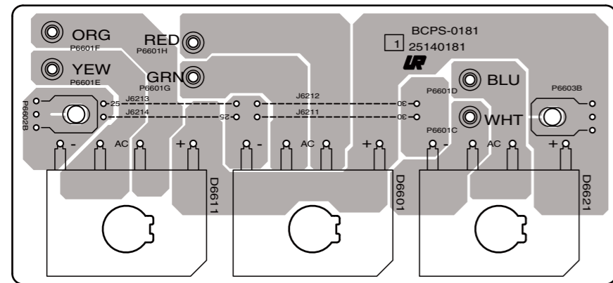
U0011 DIODE PC BOARD (BAPS-0181) Component side view from soldering side
