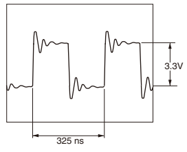
(WF05) SAI_SLCK/DIR_BCK (SD-12:F8)
