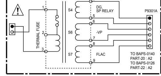
Small Transformer NPT-1582
