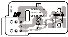
Component side view from soldering side
