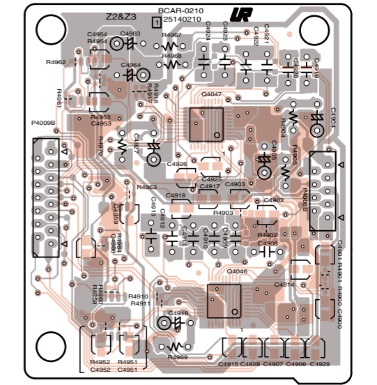
Component side view from soldering side
