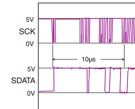
SCK/SDATA waveform (WF61) SD-14:F4,I4 SD-16:F4,I4
