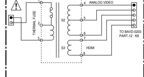
Small Transformer NPT-1582
