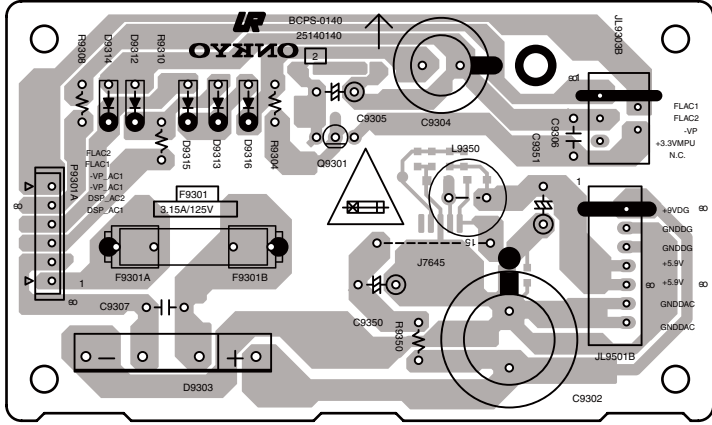
Component side view from soldering side
