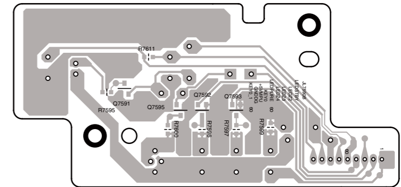
U0051 SWITCH PC BOARD (BASW-0136) Soldering side view from component side
