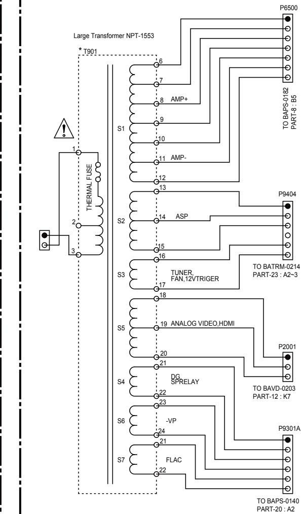
TX-NR1007/NA1007, DTR-70.1 Transformer
