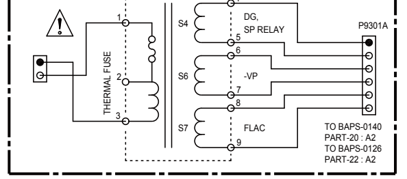
Small Transformer NPT-1582
