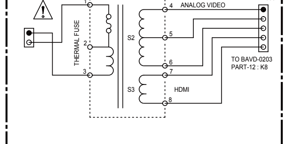
Small Transformer NPT-1582
