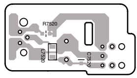
Soldering side view from component side
