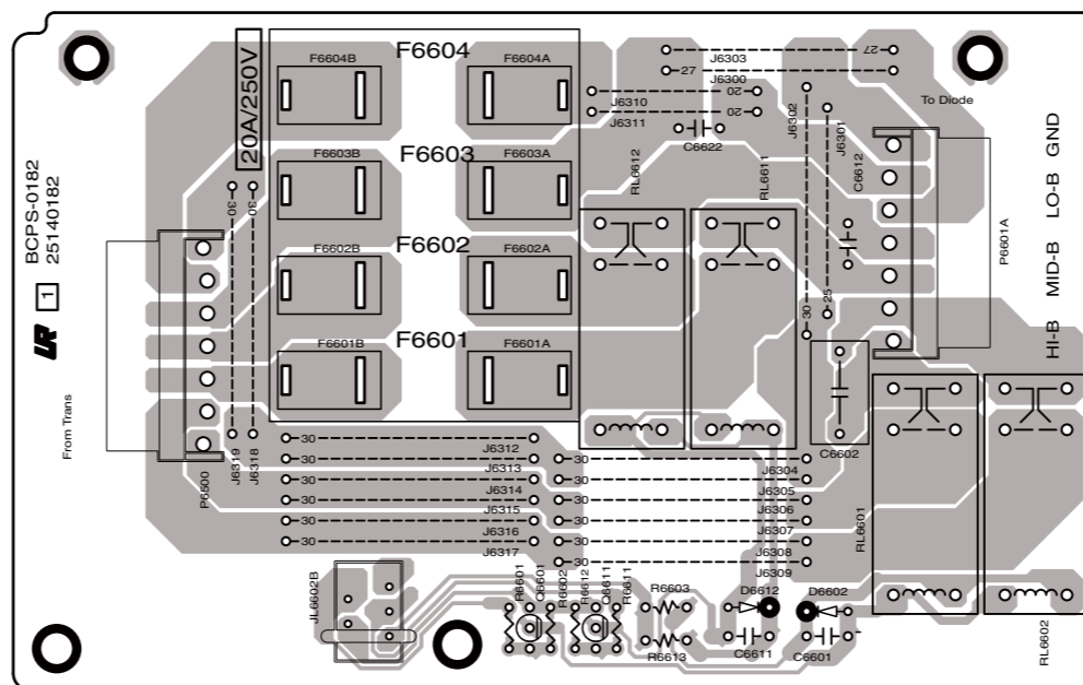
U0012 RELAY PC BOARD (BAPS-0182) Component side view from soldering side
