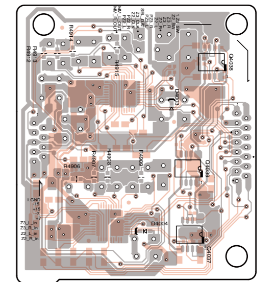
Soldering side view from component side
