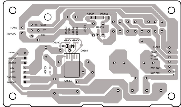
Soldering side view from component side
