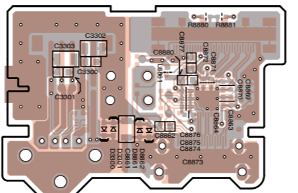
Soldering side view from component side
