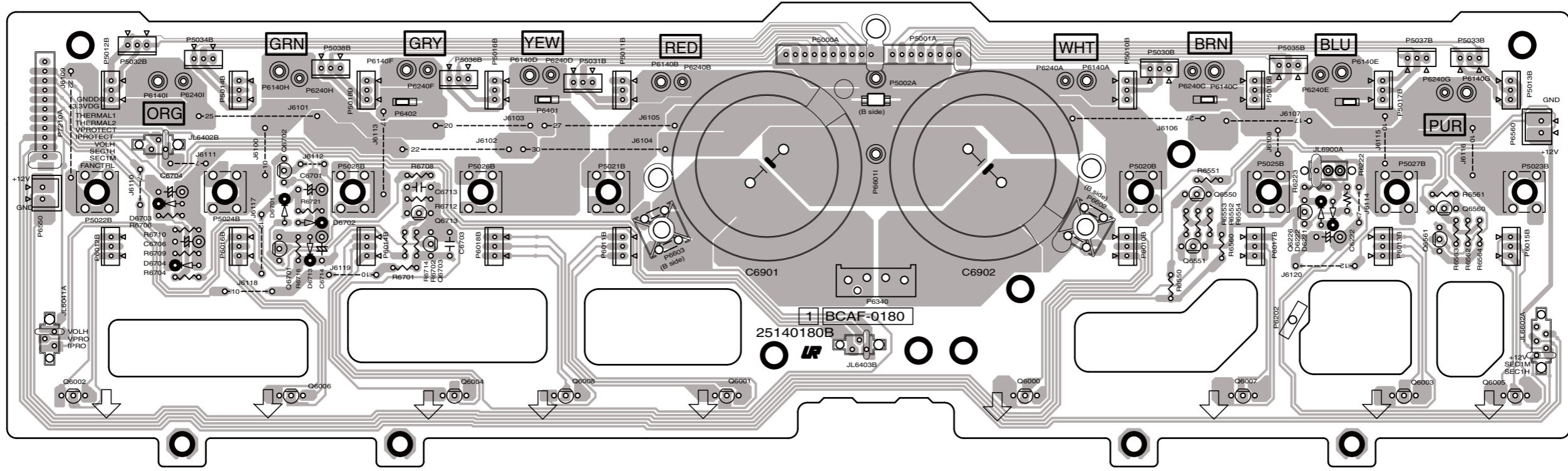
U0010 POWER SUPPLY PC BOARD (BAAF-0180) Component side view from soldering side
