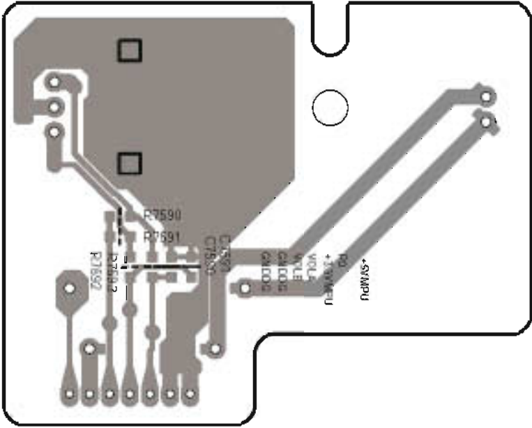
Component side view from soldering side
