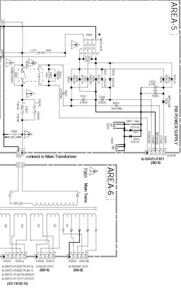
U0021 PRIMARY POWER SUPPLY PC BOARD BAPS-0084-1G-1H
