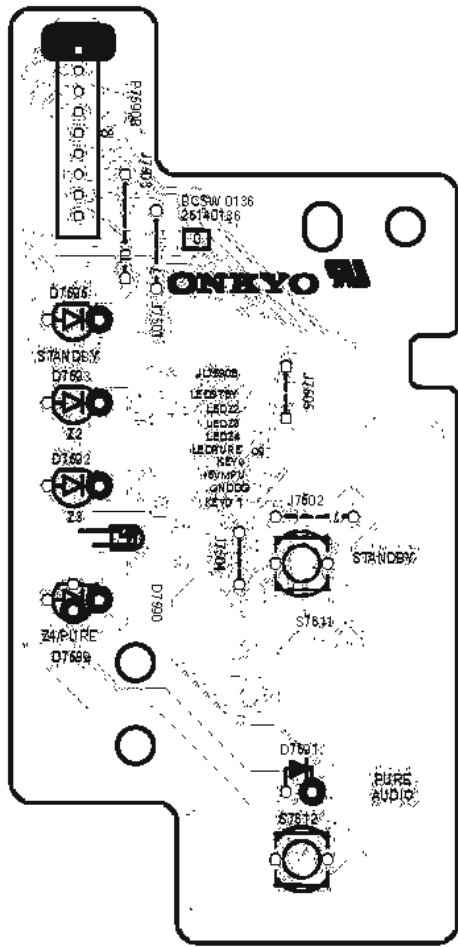
Component side view from soldering side
