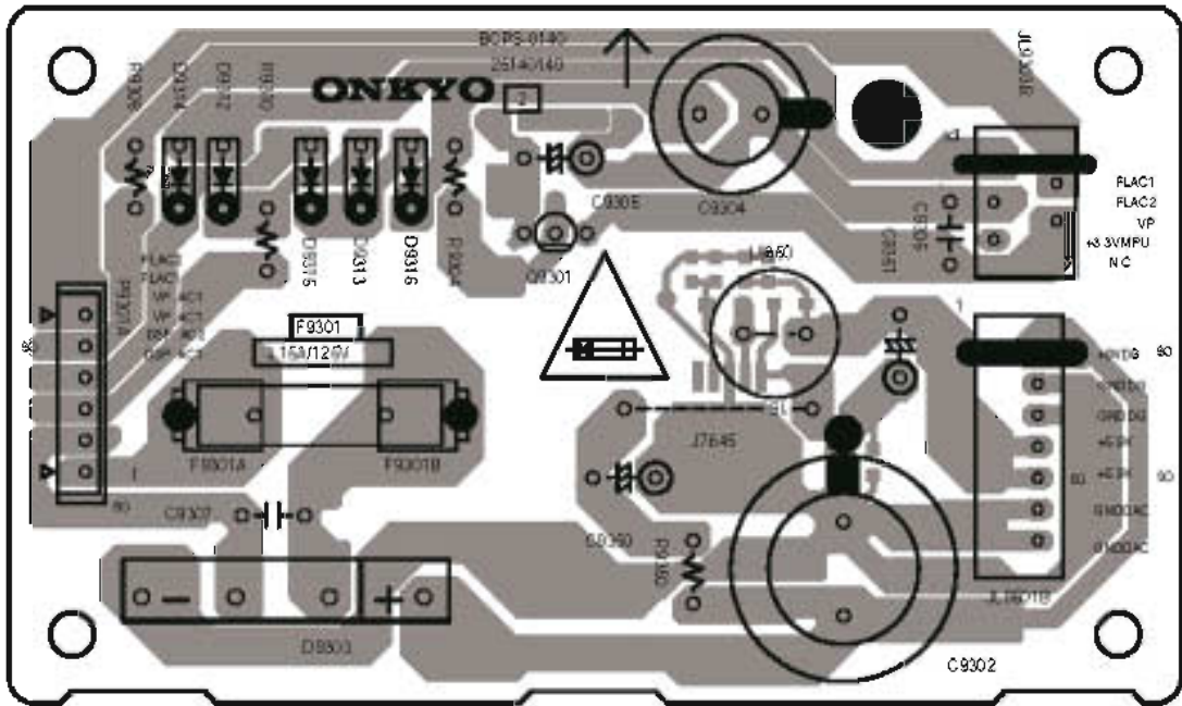
Component side view from soldering side
