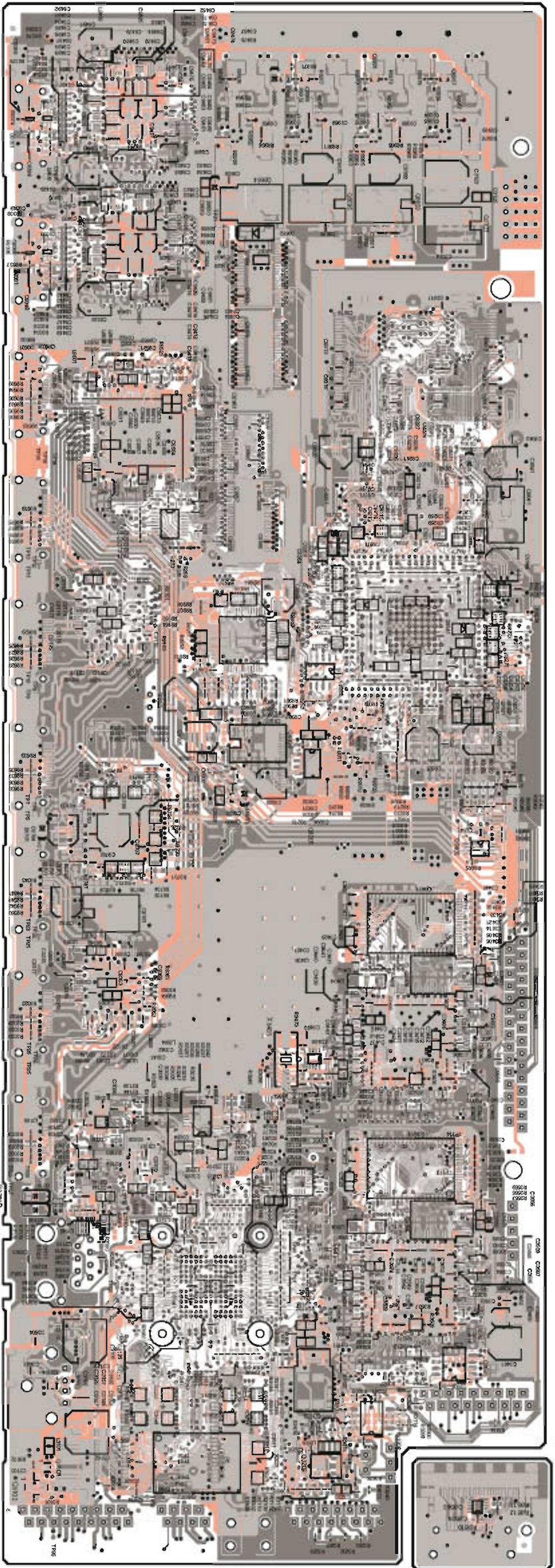
B-side view
