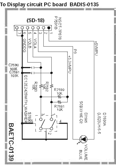
U0044 VOLUME LED PC BOARD BAETC-0139-1A
