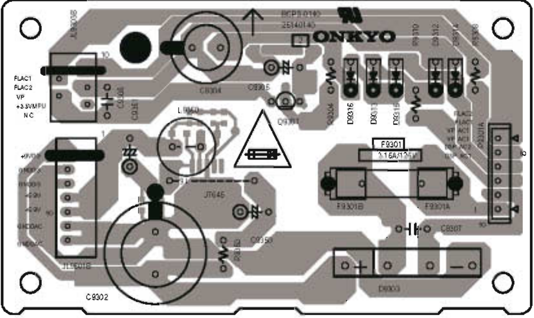
Soldering side view from component side
