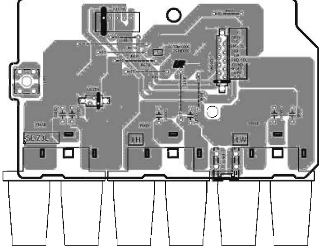
U0022 SPEAKER TERMINAL-2 PC BOARD BATRM-0085
