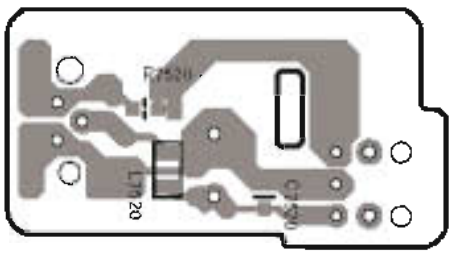
Soldering side view from component side
