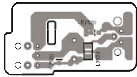
Component side view from soldering side
