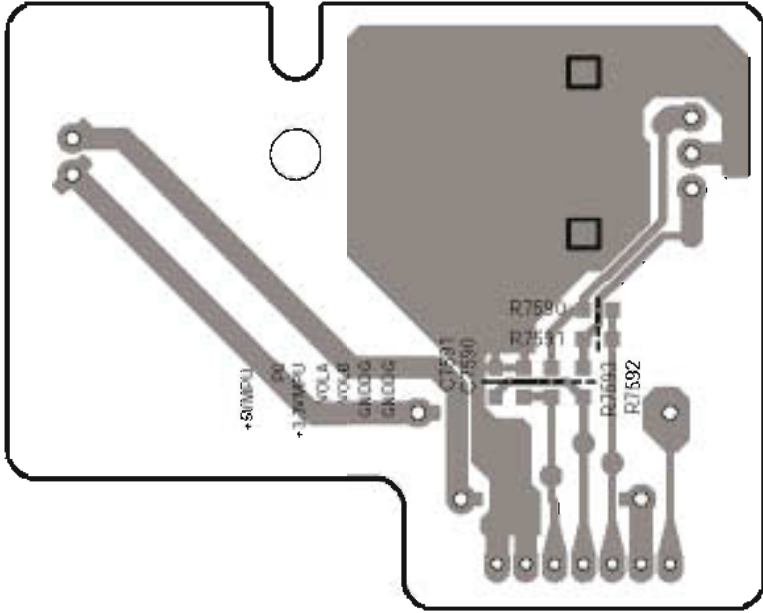
Soldering side view from component side
