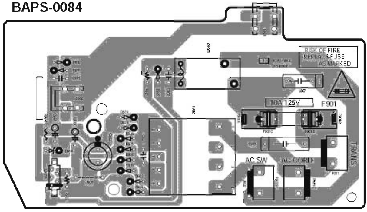
Soldering side view
