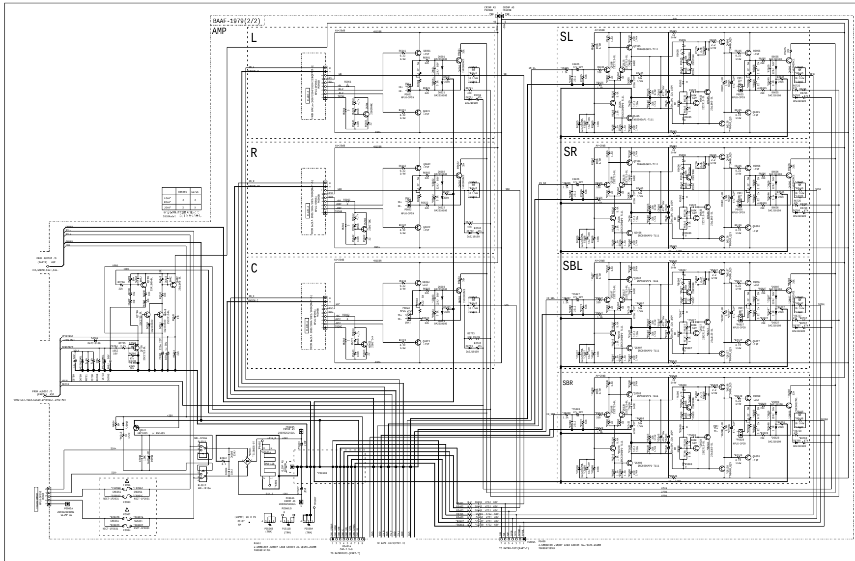
MODELNO.TX-NR555/656/757,TX-RZ610/710/810,HT-R695,DRX-2/3/4/5 SCHEMATIC DIAGRAM (PART-4) AMP SECTION
