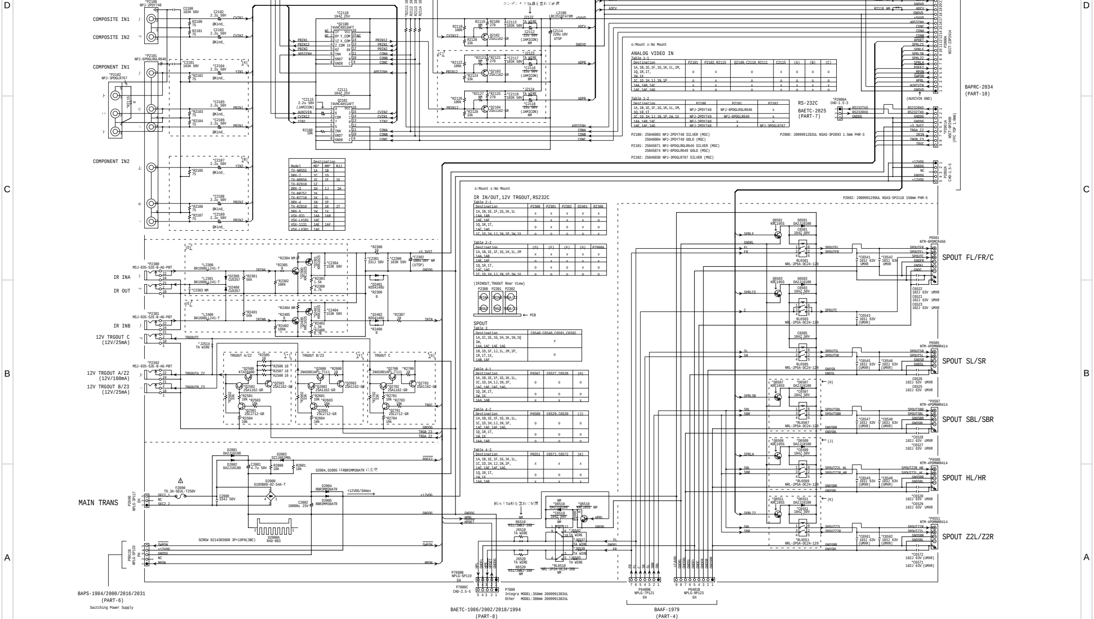
MODEL NO. TX-NR555/656/757, TX-RZ610/710/810, HT-R695, DRX-2/3/4/5 SCHEMATIC DIAGRAM(PART-7) VIDEO, SPOUT, IR/12VTRG SECTION
