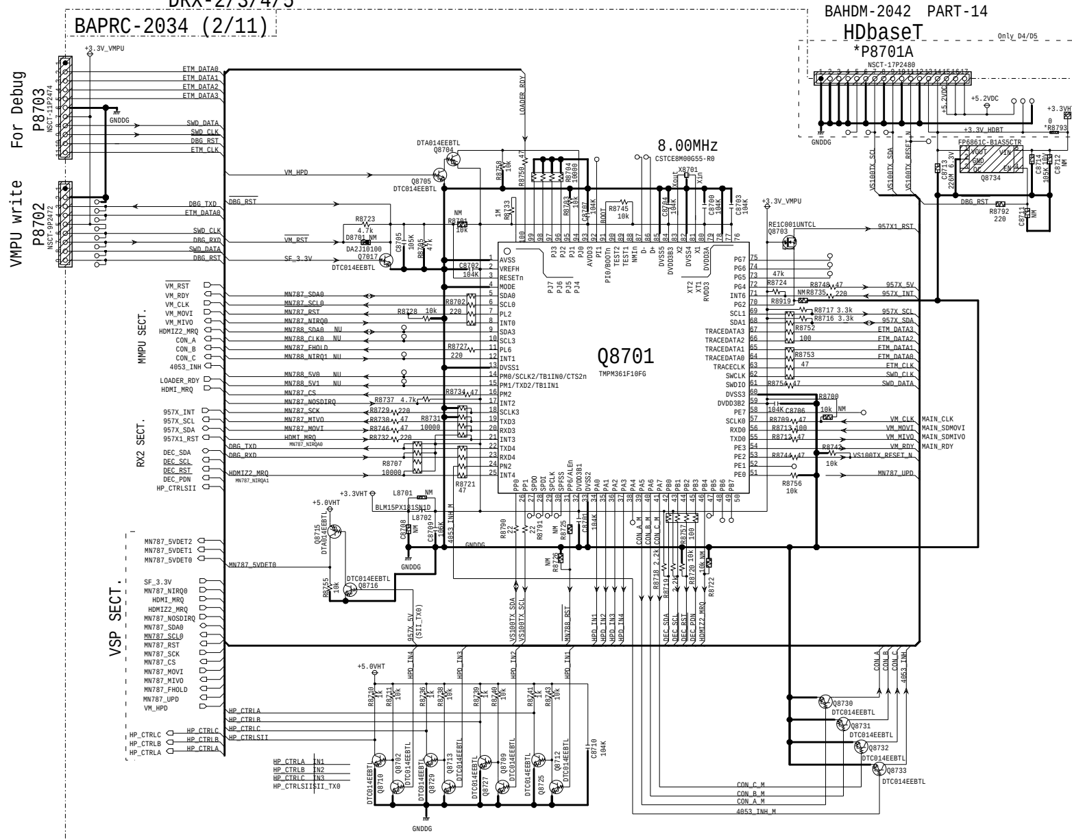
SCHEMATIC DIAGRAM (PART-10) VMPU SECTION
