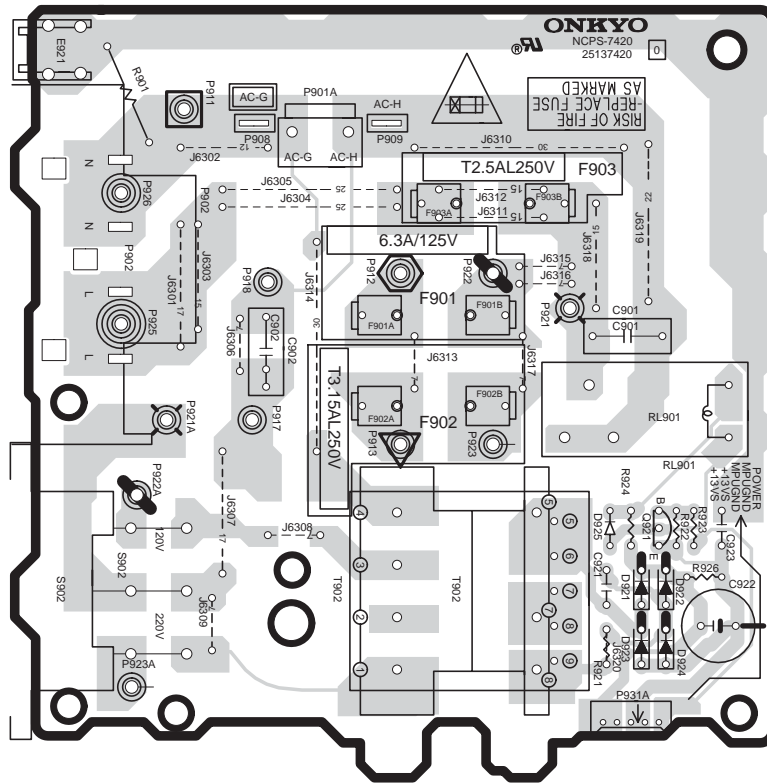
NAPS-7420, Primary circuit PC board
