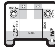
NASW-7418, Power switch PC board (Except 120V model)
