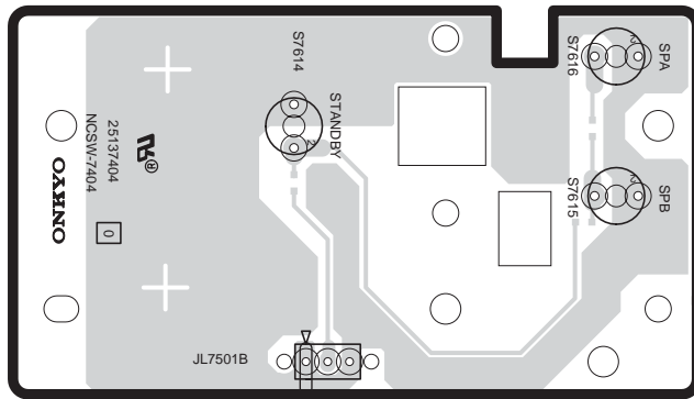
Component side
