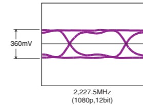
HDMI D0,D1,D2 waveform (WF41) PART-11:B3, H4
