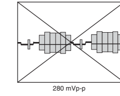
S-Video C waveform (WF23)
