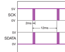
SCK/SDATA waveform (WF61) PART-9:F4/D4
