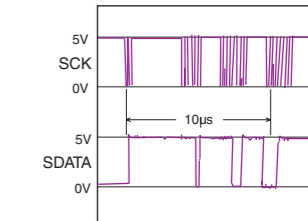
SCK/SDATA waveform (WF61) PART-9:F4/D4
