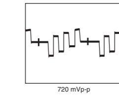
Component PB waveform (WF25) PART-6:B4,B5
