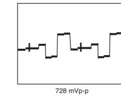
Component PR waveform (WF26) PART-6:B4
