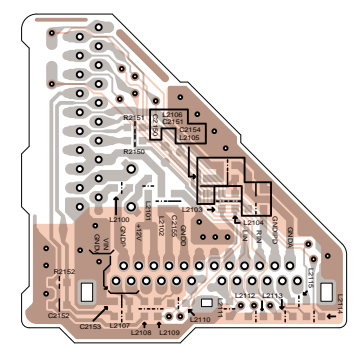
U0022 UNIVERSAL PORT PC BOARD (BAETC-0027)
