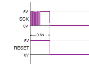
SCK/RESET waveform (WF63) PART-9:F4/D4
