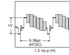
Composite waveform (WF21) PART-6:B7
