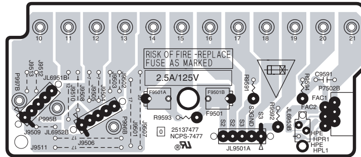
U17 Secondary circuit PC board
