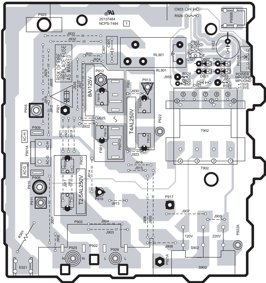
U24 Primary circuit PC board
