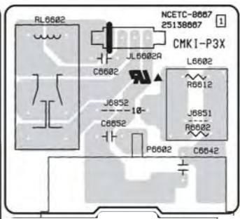
U042 NAPS-8665, Secondary circuit PC board
