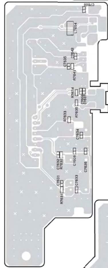
NAETC-8662, Front video PC board
