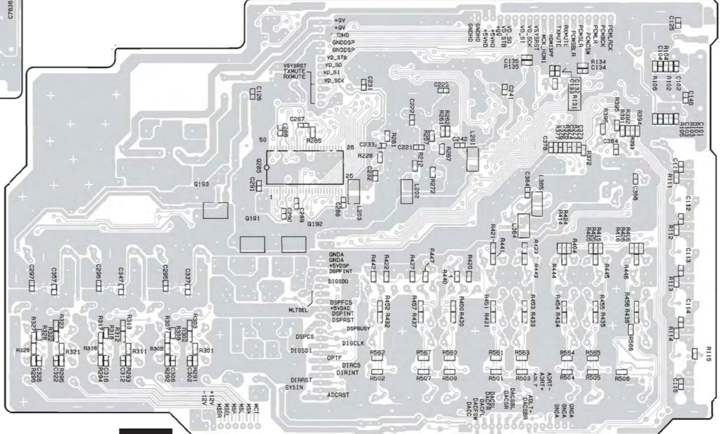
NADG-8660, DSP circuit PC board
