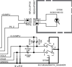
U020 Volume illuminate PC board BAETC-0116
