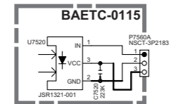
U019 AUX Input terminal PC board BAETC-0115
