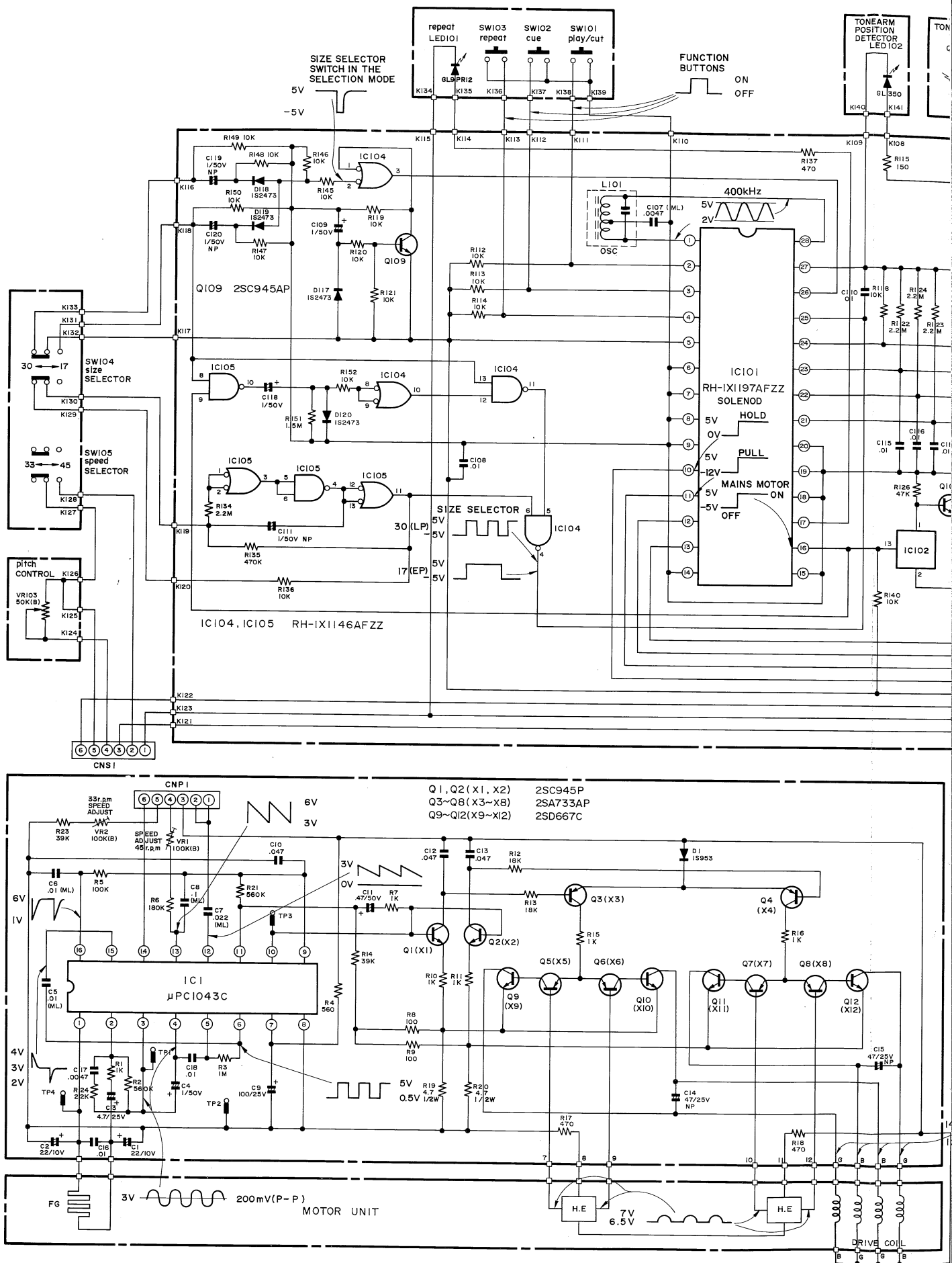
Figure 11 SCHEMATIC DIA
