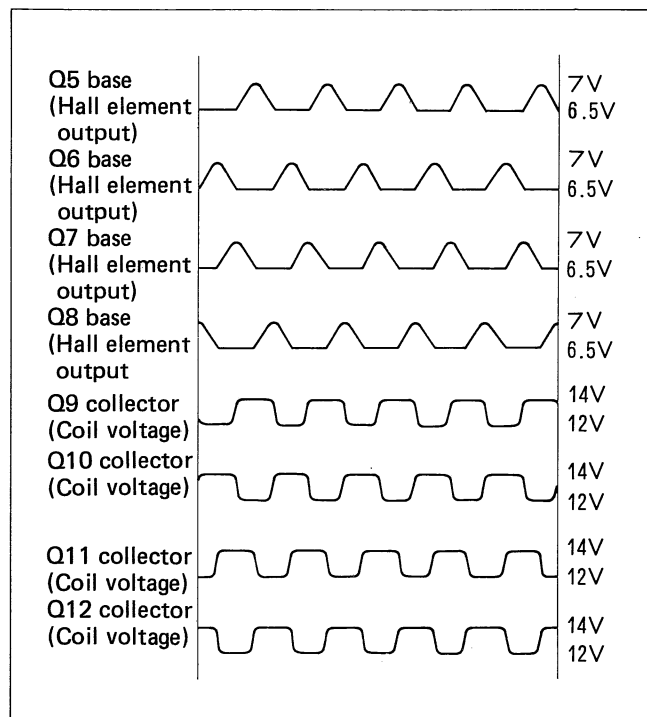
Figure 7-2 WAVEFORMS OF MOTOR DRIVE CIRCUIT
