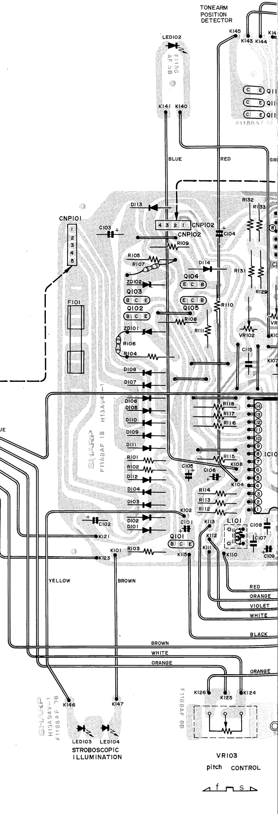
Figure 13 WIRING SIDE OF PRINTED V
