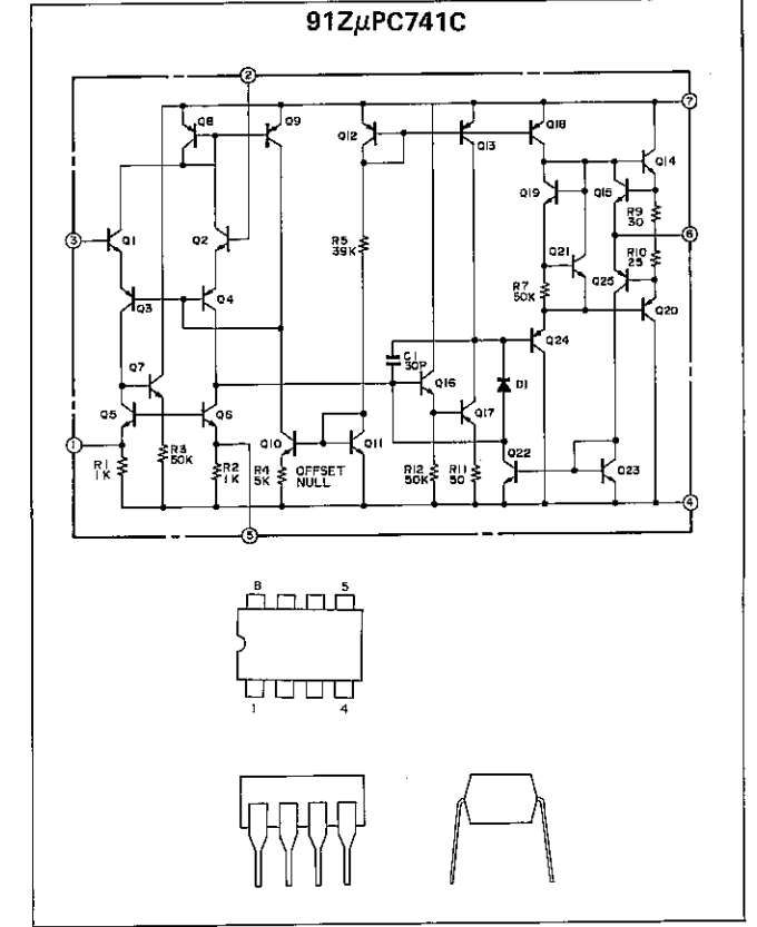
Figure 47 EQUIVALENT OF INTEGRATED CIRCUIT (IC301)
