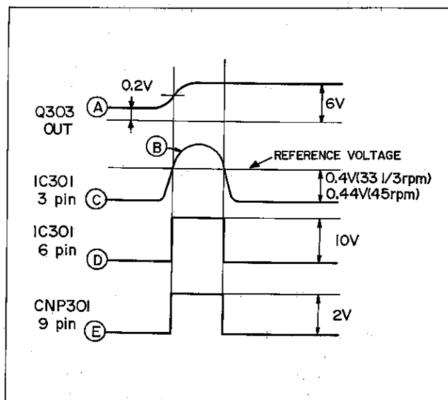
Figure 33 TIME CHART
