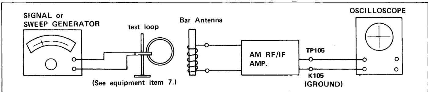
Figure 29 AM RF ALIGNMENT EQUIPMENT CONNECTIONS
