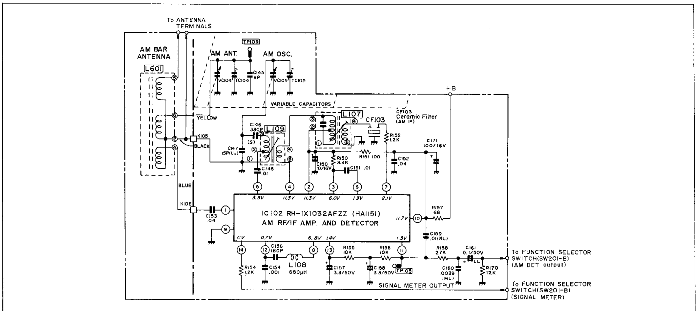
Figure 20 AM CIRCUIT
