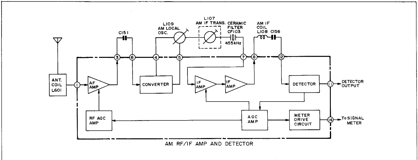
Figure 19 BLOCK DIAGRAM OF IC102
