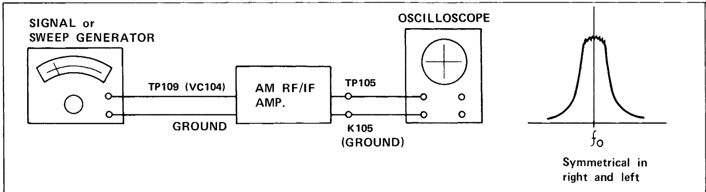
Figure 28 AM IF ALIGNMENT EQUIPMENT CONNECTIONS
