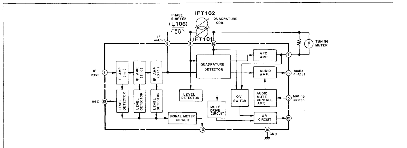
Figure 11 BLOCK DIAGRAM OF IC101
