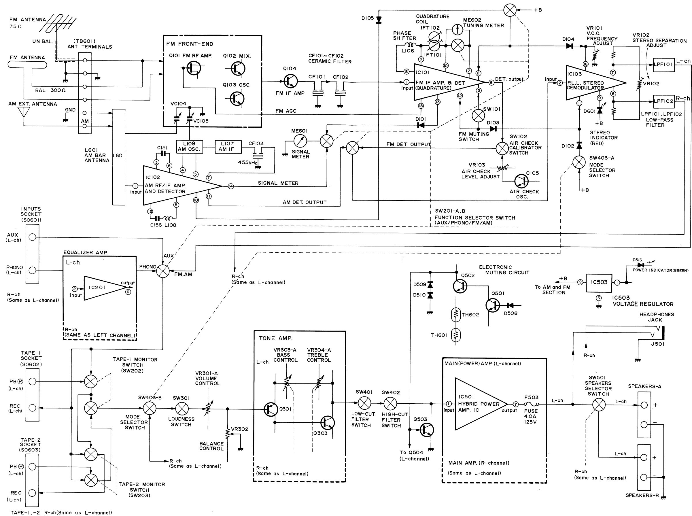
Figure 5 BLOCK DIAGRAM
