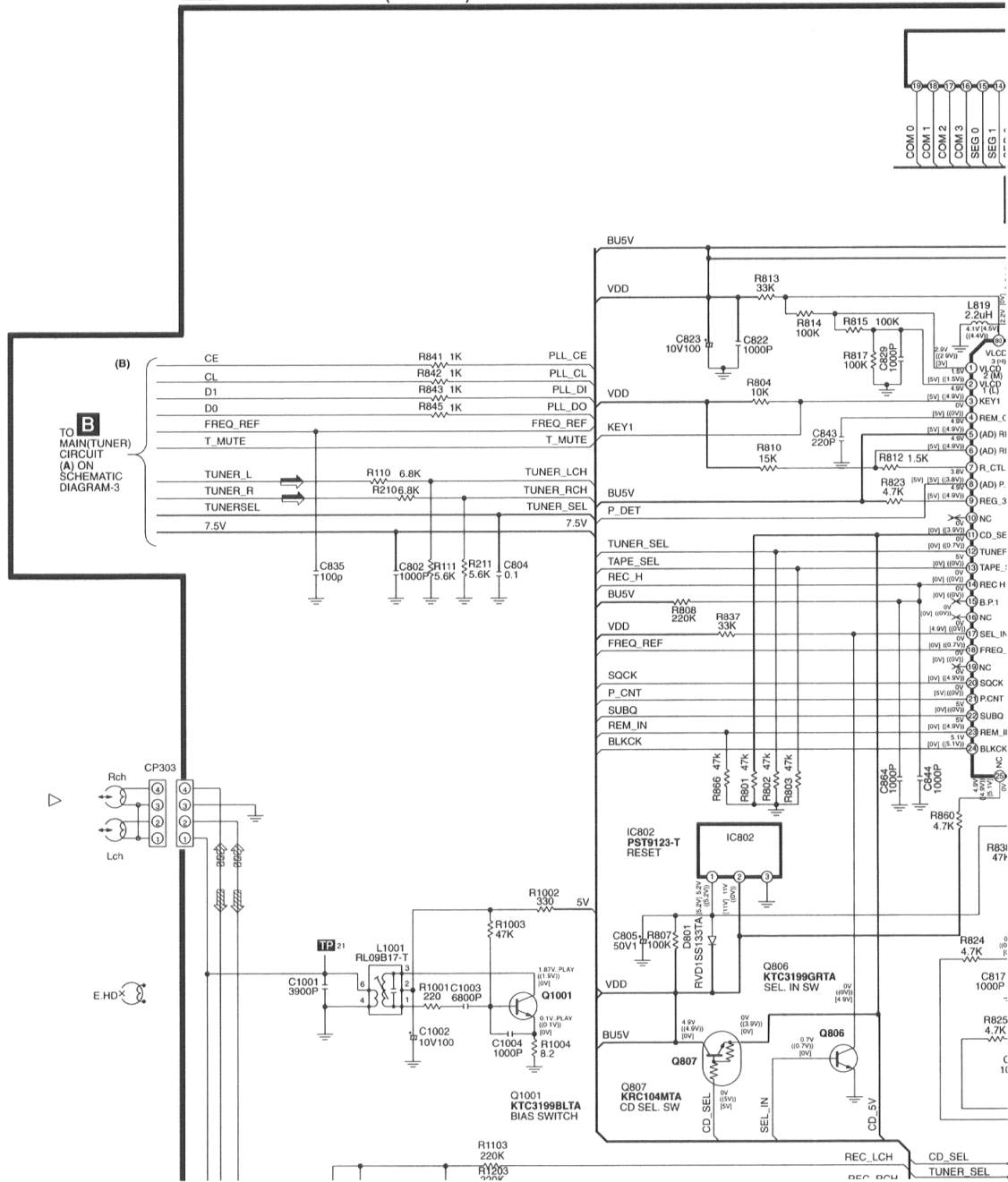
SCHEMATIC DIAGRAM-4
