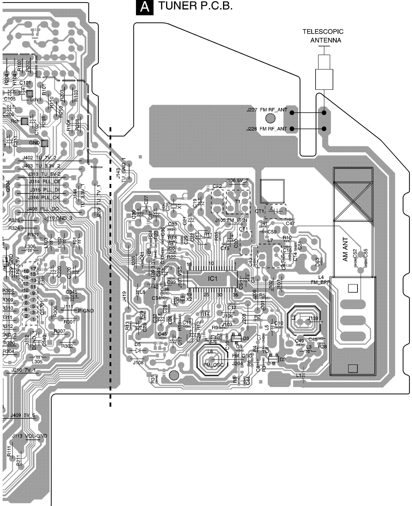
RX-CD29 TUNER &amp; MAIN P.C.B.
