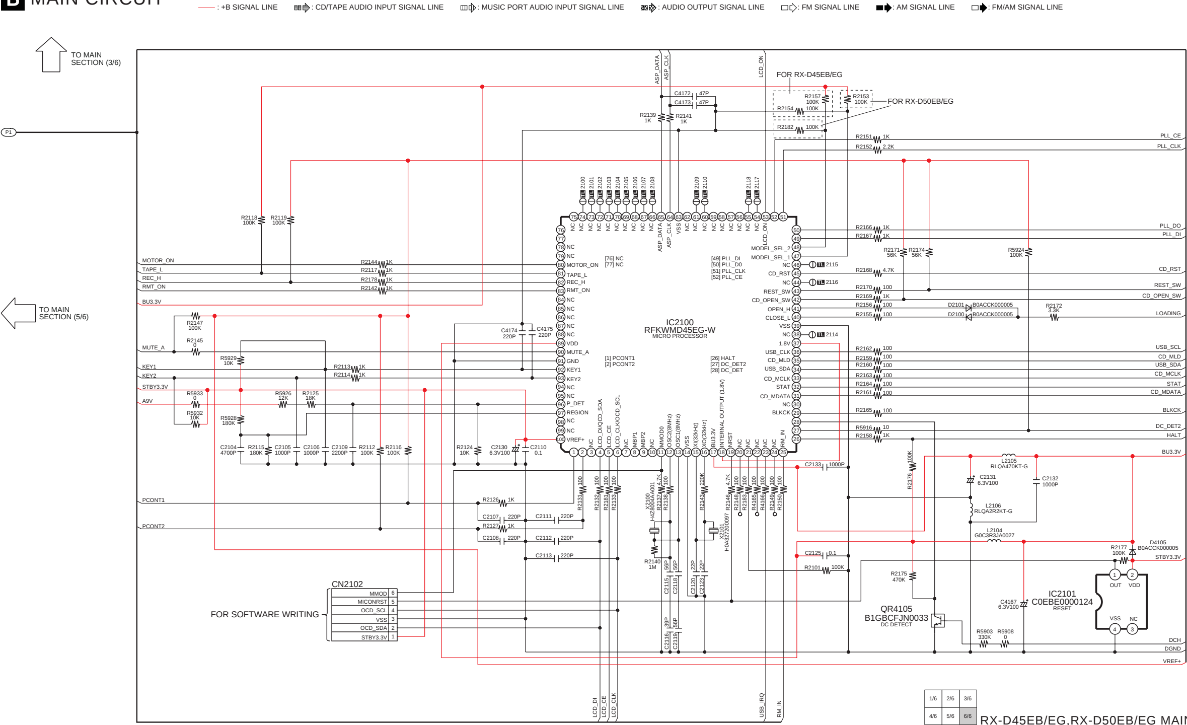
SCHEMATIC DIAGRAM - 7
