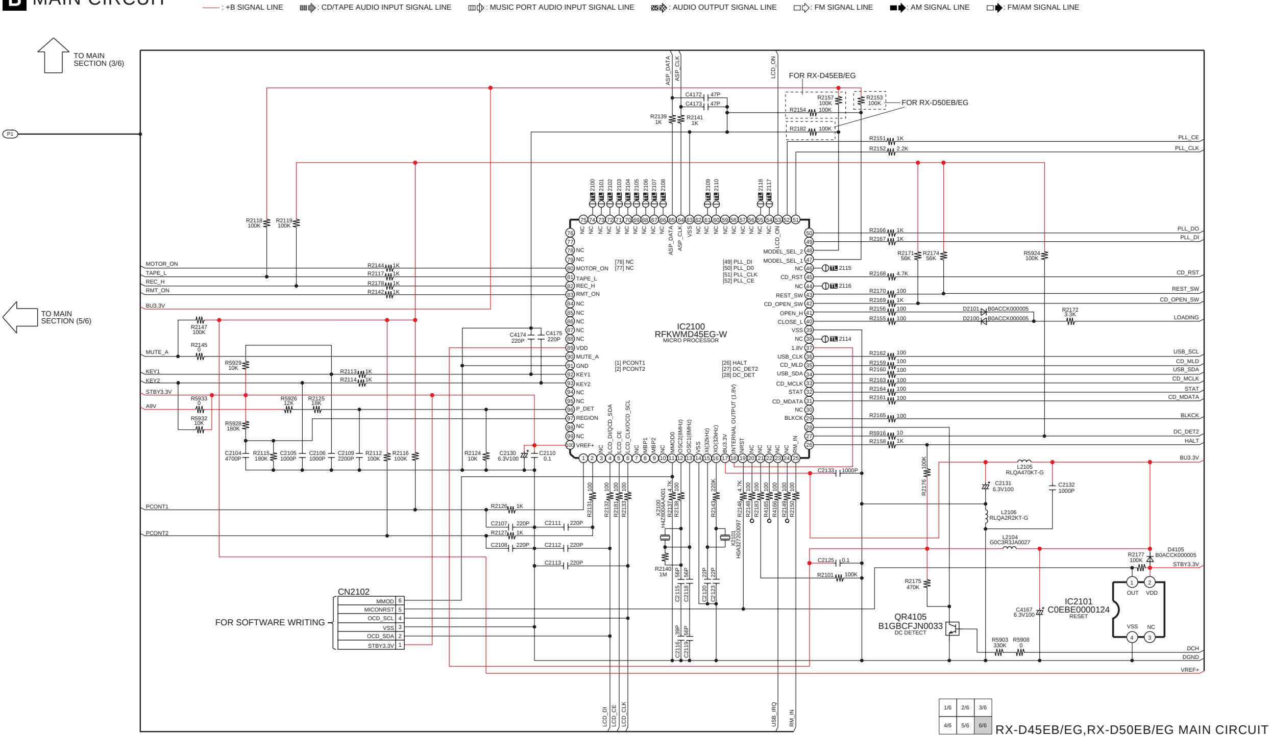
SCHEMATIC DIAGRAM - 7
