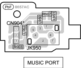
J MUSIC PORT P.C.B. (REPNT0061BA...RX-D50EG ONLY) (REPNT0061HA...RX-D50EB ONLY)
