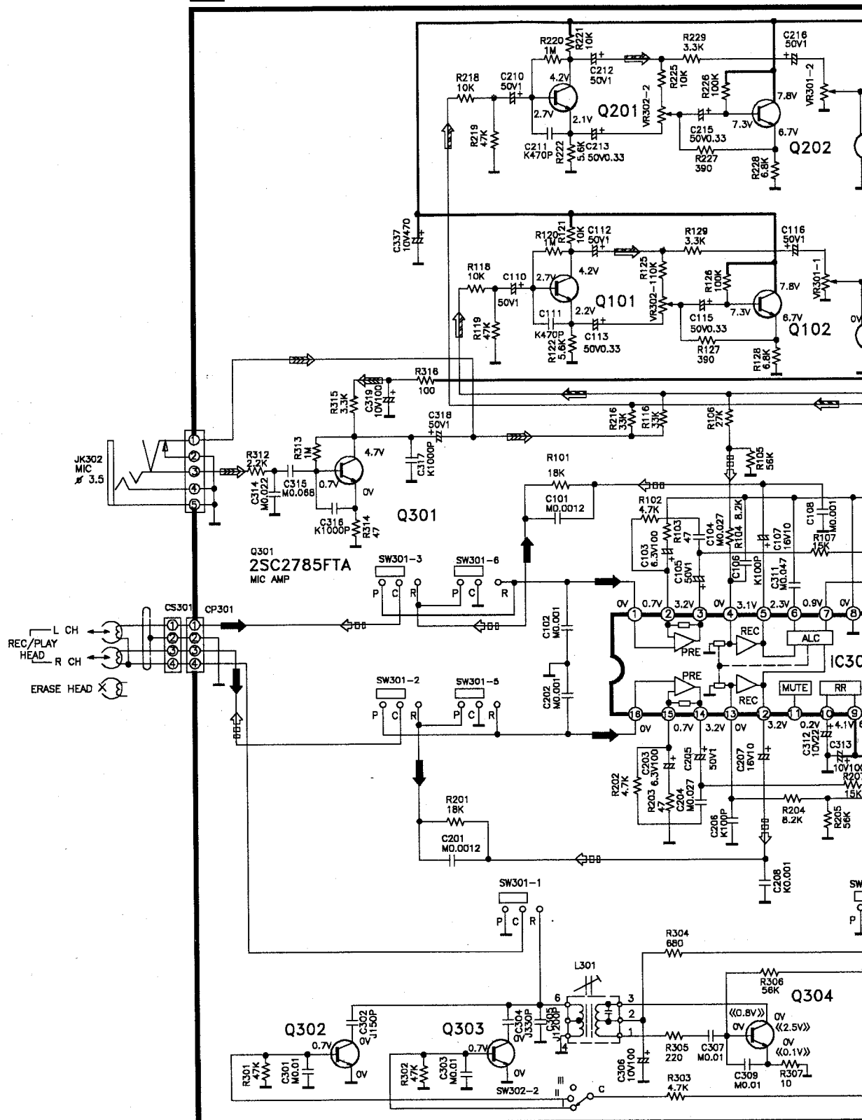
B MAIN CIRCUIT
