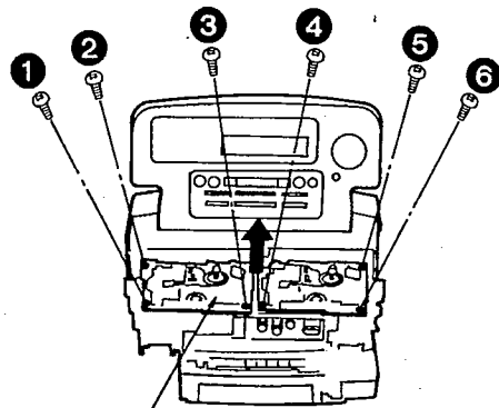
Mechanism unit
