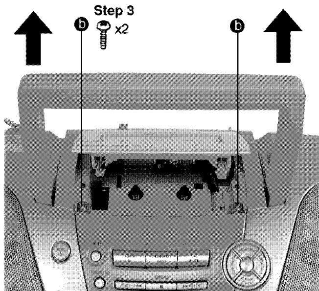
Step 3: Remove the two screws and lift up the front cabinet.
