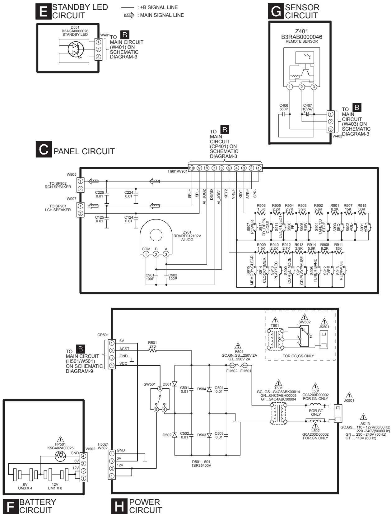
SCHEMATIC DIAGRAM-14
