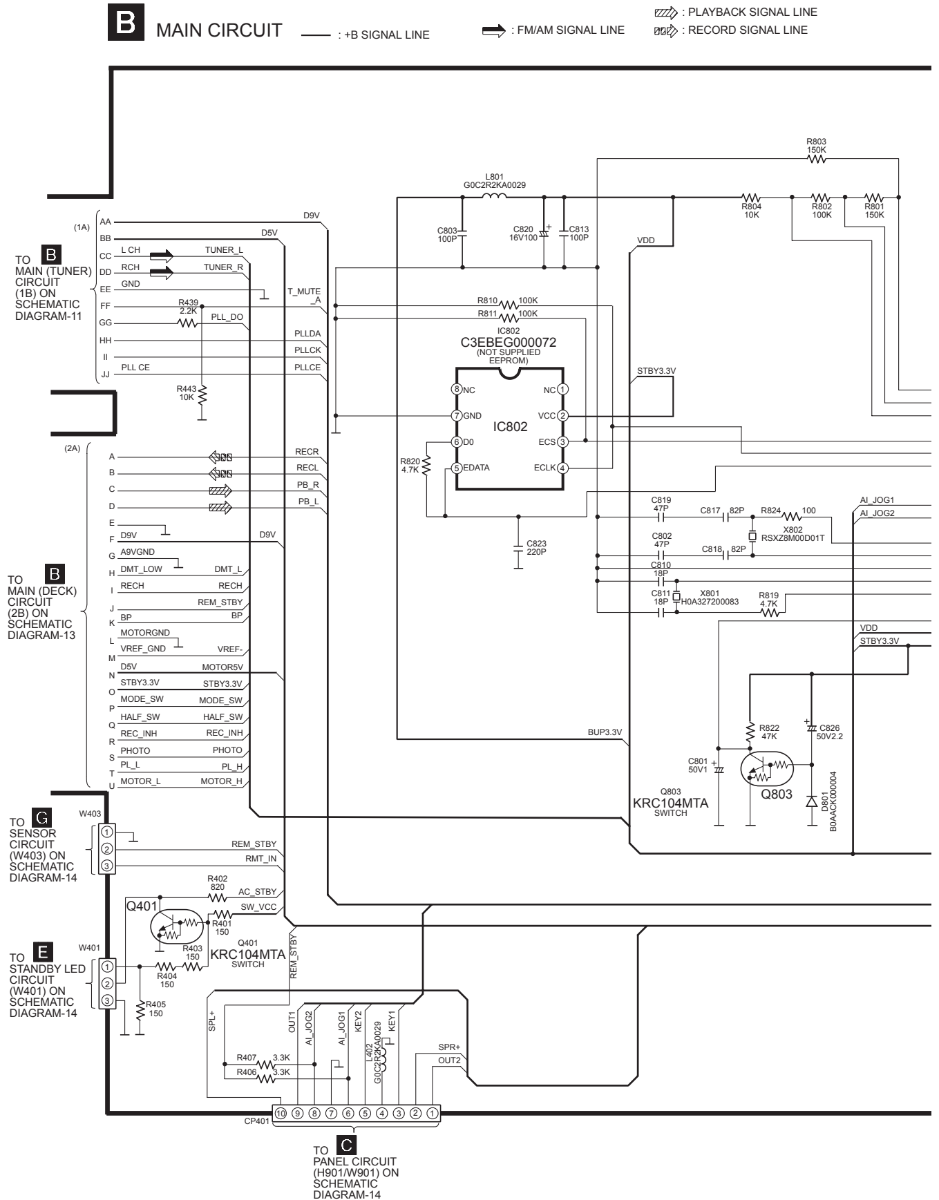
SCHEMATIC DIAGRAM-3
