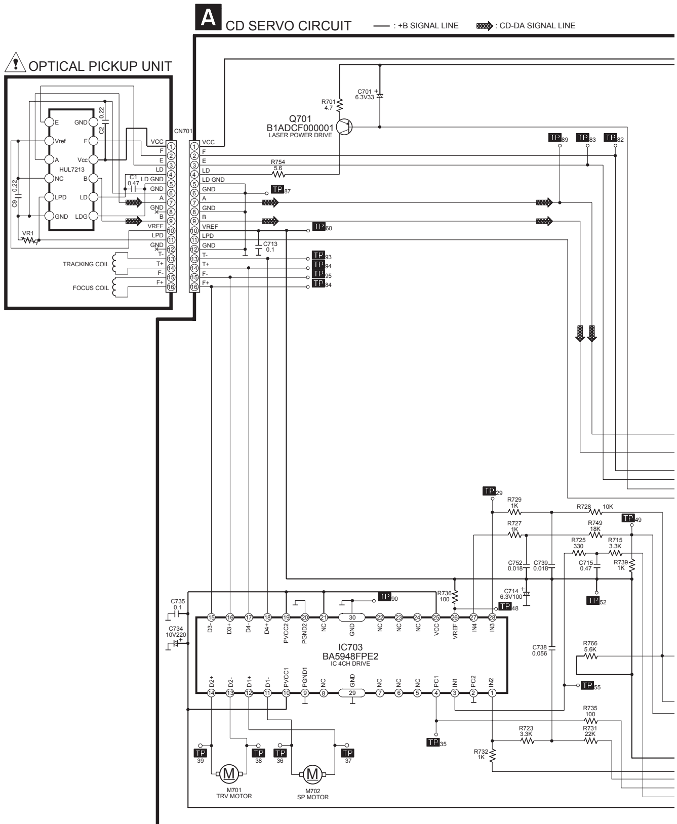
SCHEMATIC DIAGRAM - 1
