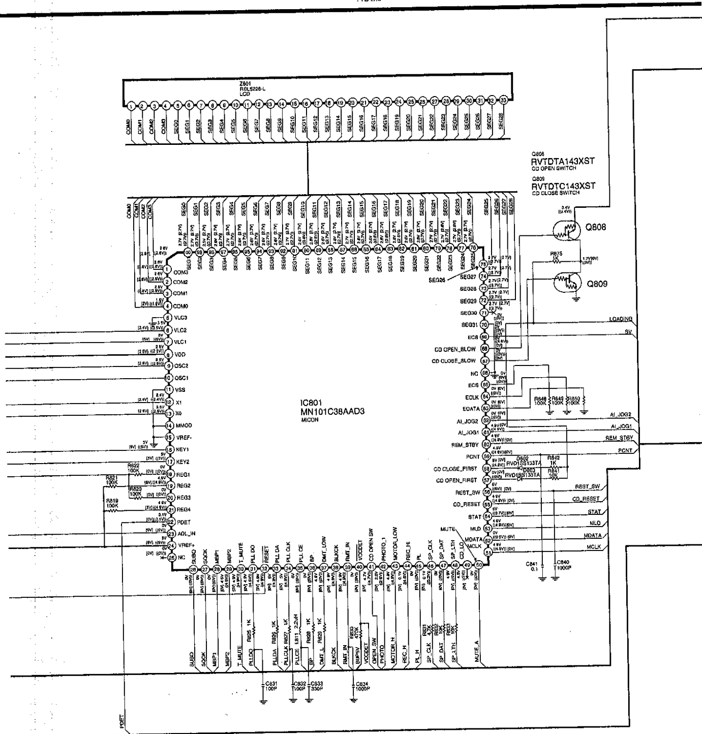
Schematic Diagram-6
