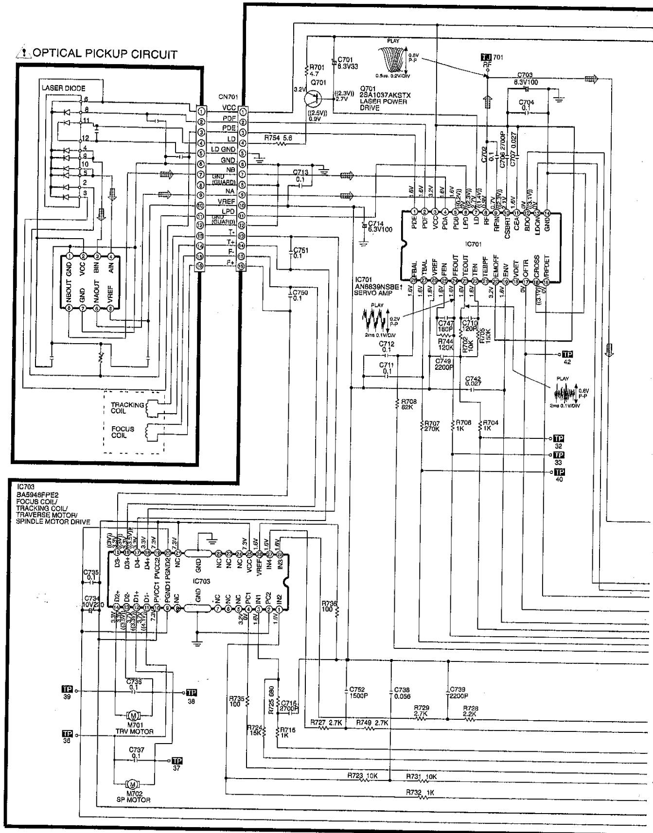
SCHEMATIC DIAGRAM-1
