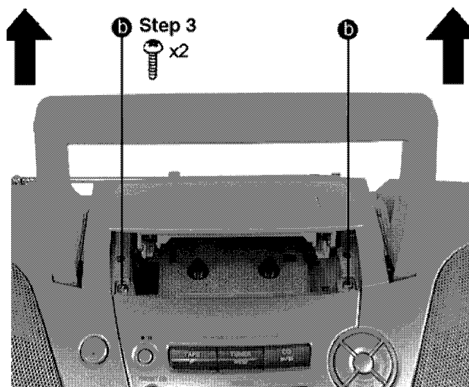
Step 3: Remove the two screws and lift up the front cabinet.
