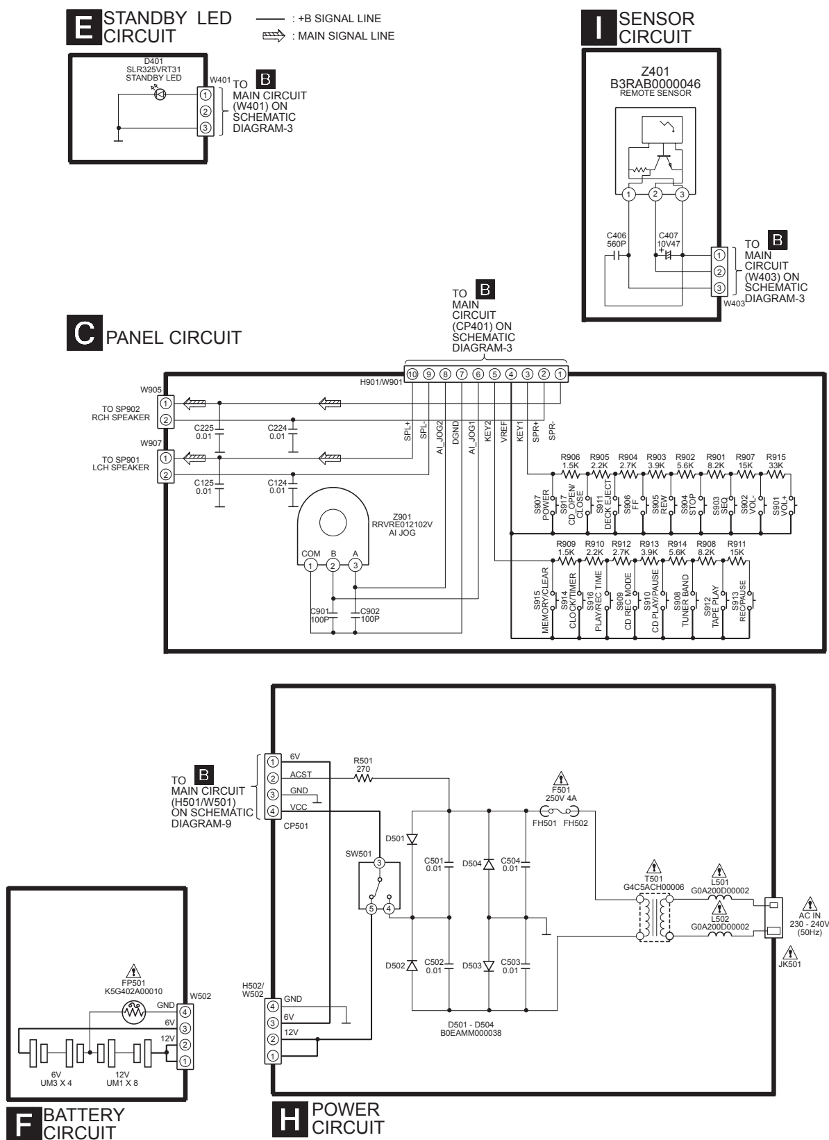
SCHEMATIC DIAGRAM-14
