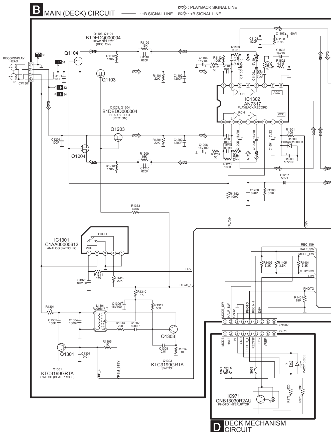
SCHEMATIC DIAGRAM-12
