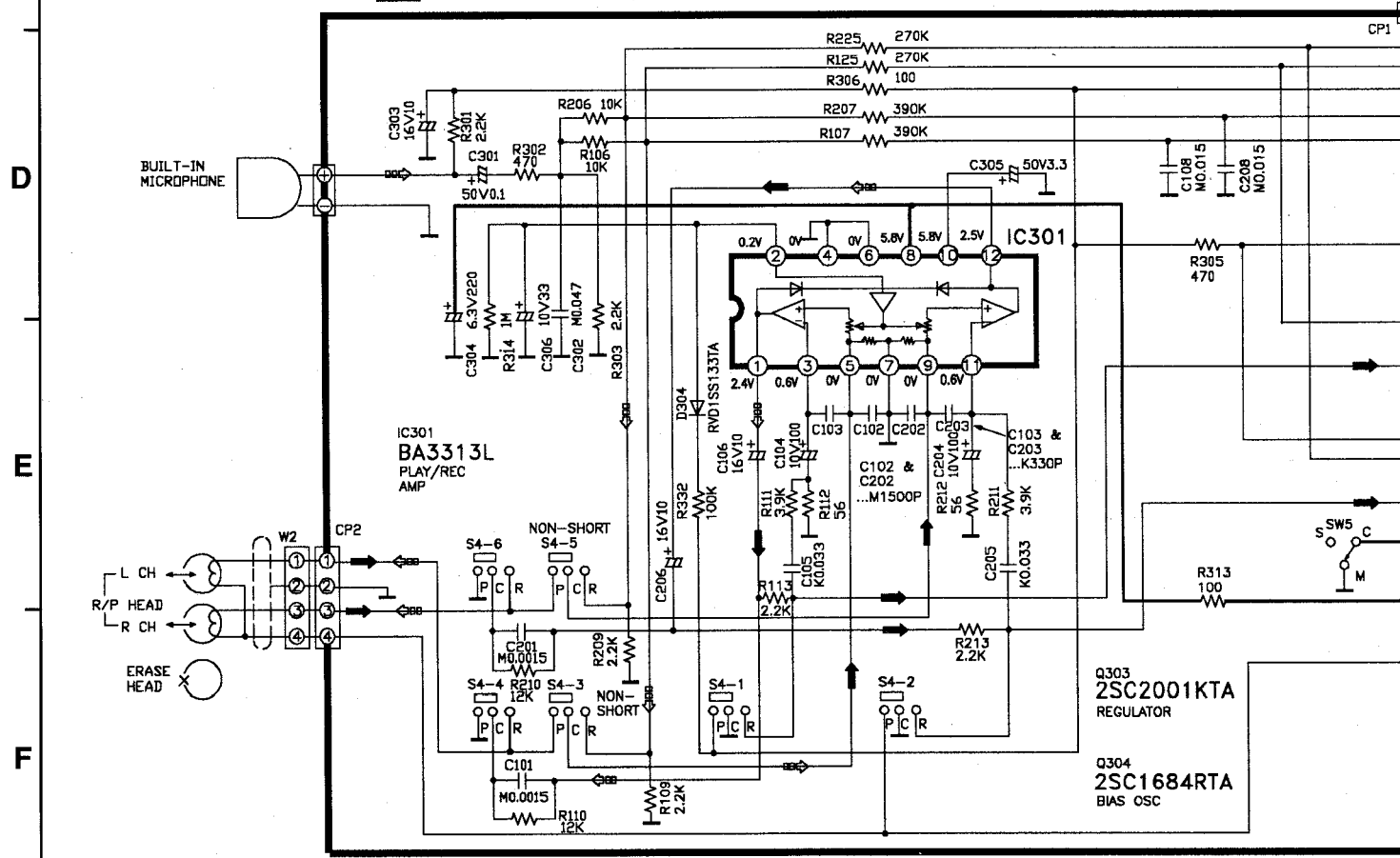
B MAIN CIRCUIT
