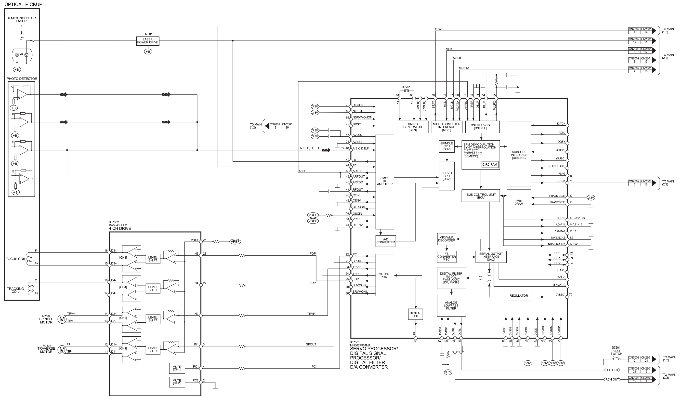
SA-AK350E/EB/EG CD SERVO BLOCK DIAGRAM
