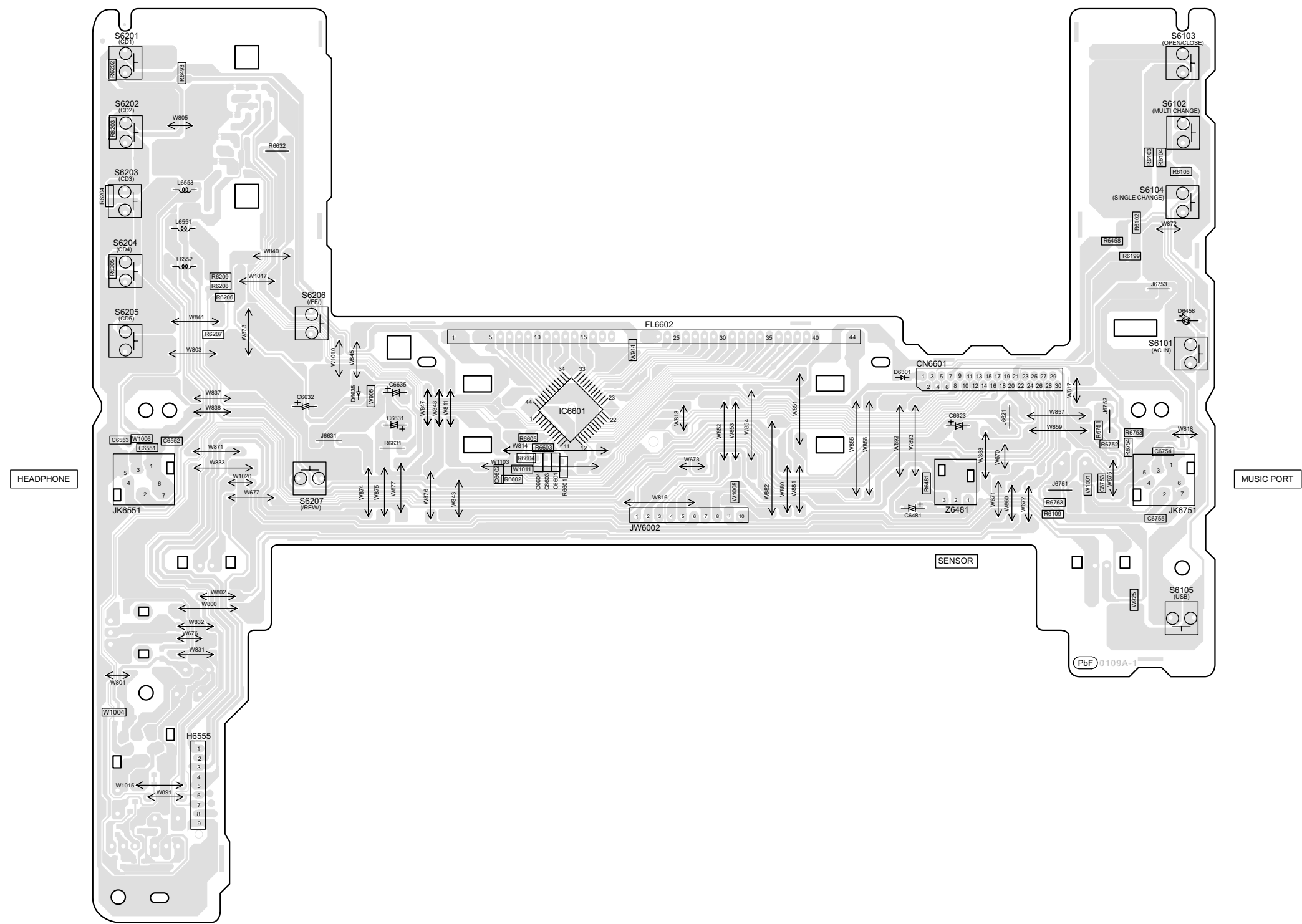
C PANEL P.C.B (REPV0131H)
