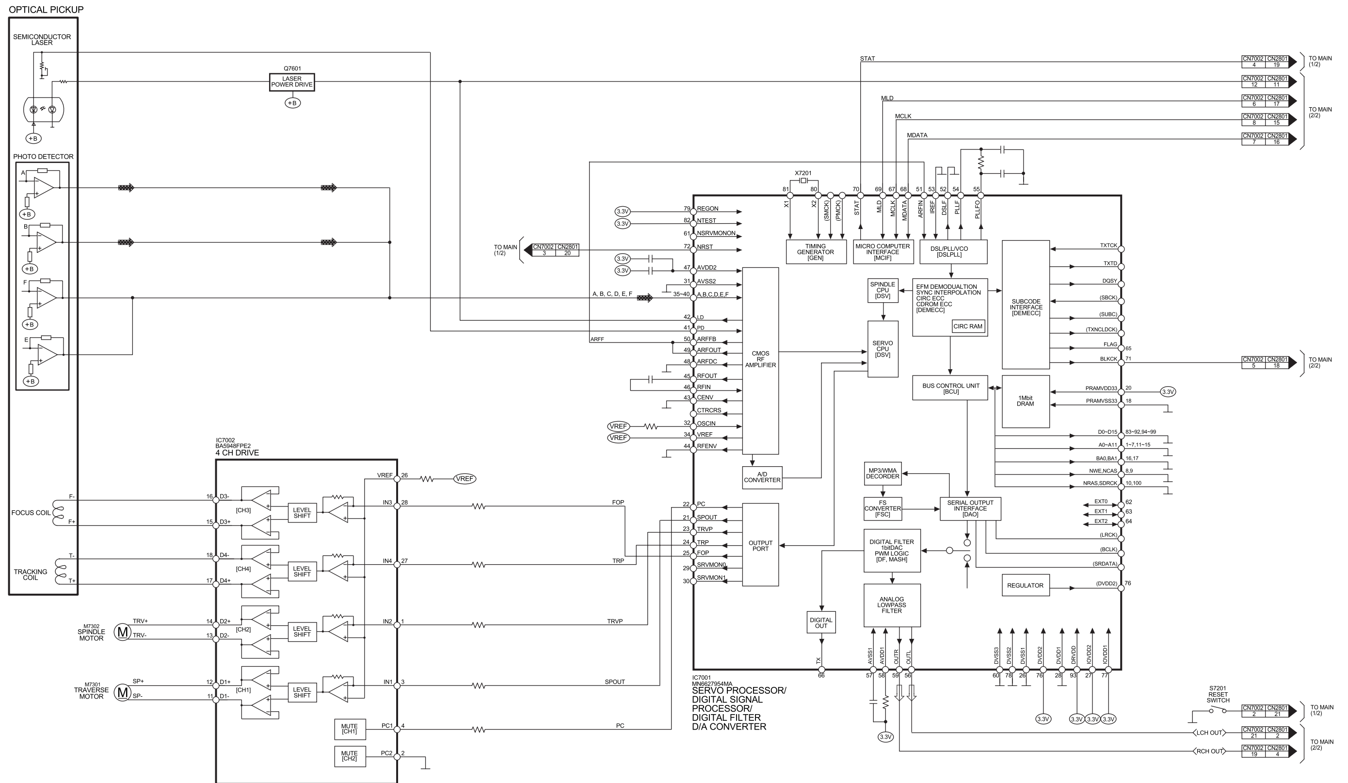
SA-AK350PL CD SERVO BLOCK DIAGRAM
