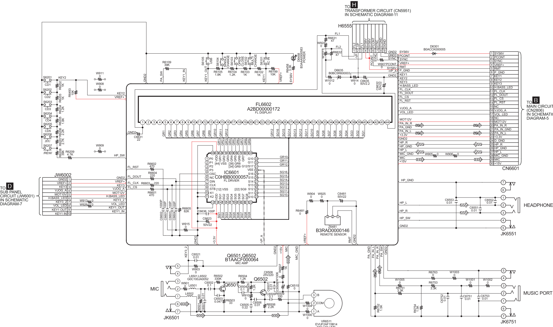
C PANEL CIRCUIT
