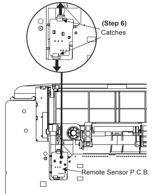
Step 7 Lift up the Panel P.C.B., Tact Switch P.C.B. & Remote Sensor P.C.B. altogether as arrow shown.
