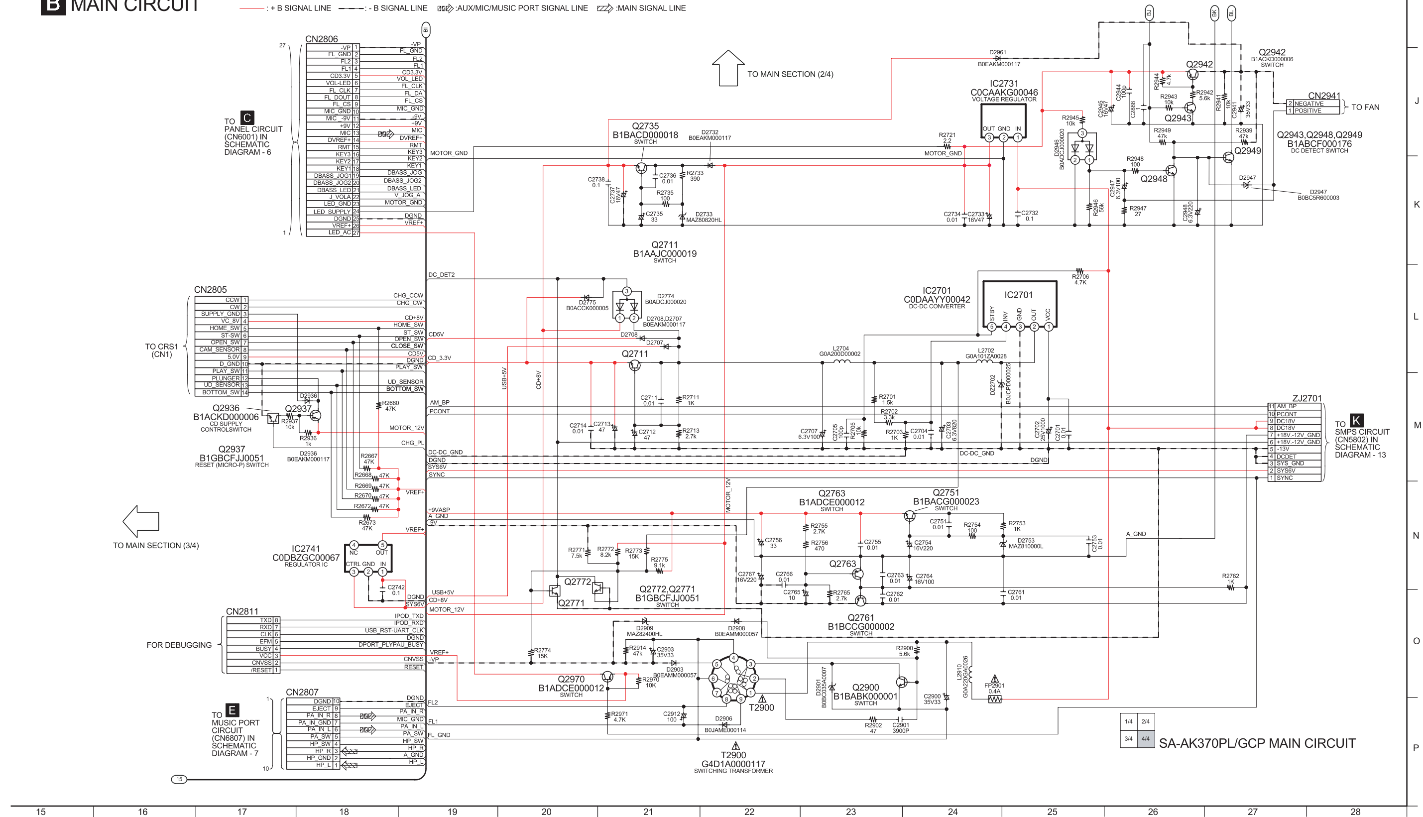
SCHEMATIC DIAGRAM - 5
