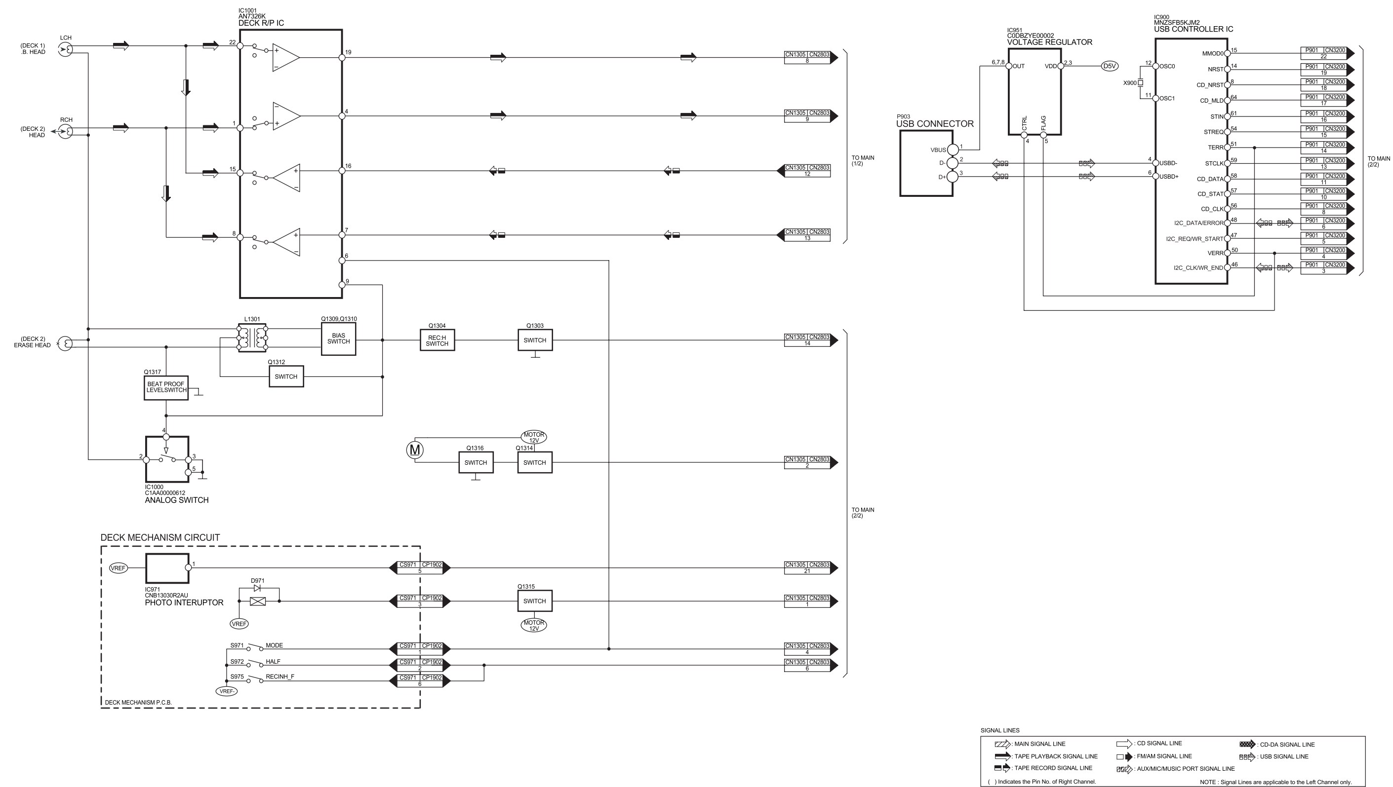
SA-AK370PL/GCP DECK/DECK MECHANISM/USB CIRCUIT BLOCK DIAGRAM
