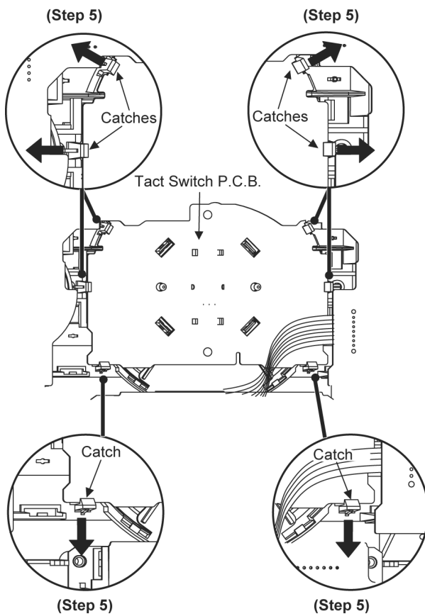
Step 5 Release 6 catches at Tact Switch P.C.B..
