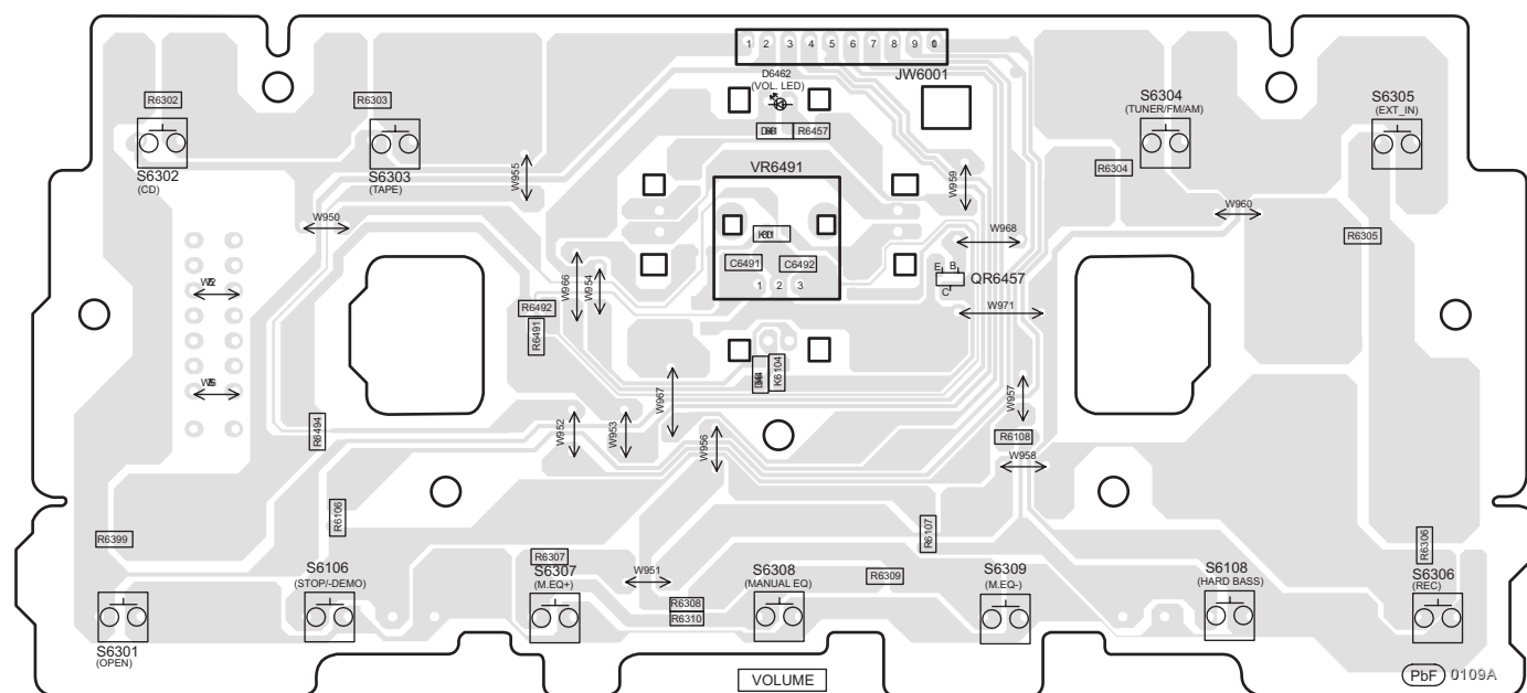
D SUB PANEL P.C.B (REPV0131E)
