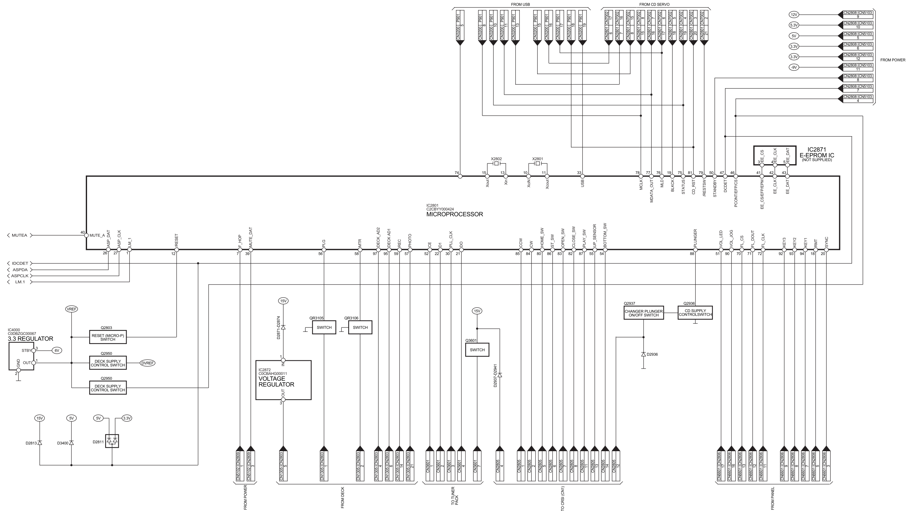
SA-AK450GCP MAIN 2/2 DIAGRAM
