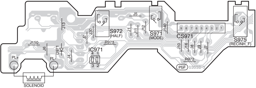
G DECK MECHANISM P.C.B (REPX0321F)
