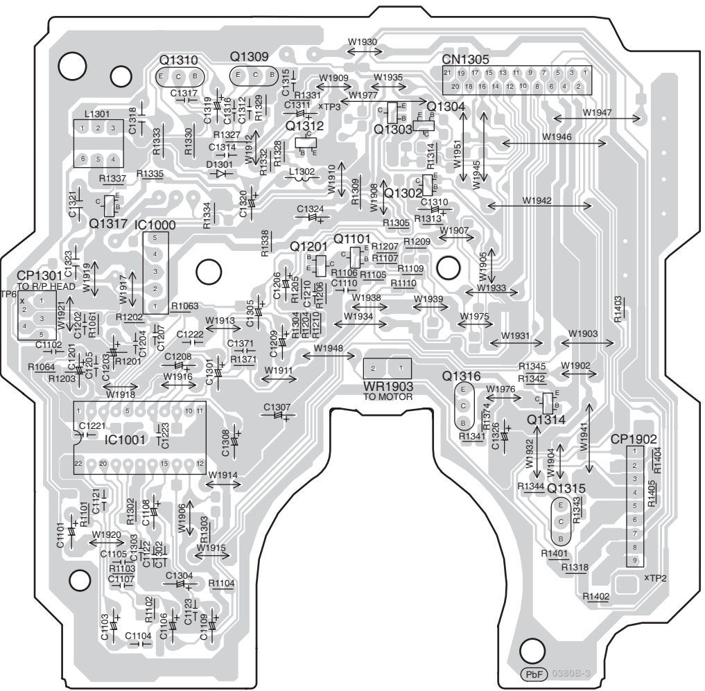
I DECK MECHANISM P.C.B (REPX0321F)
