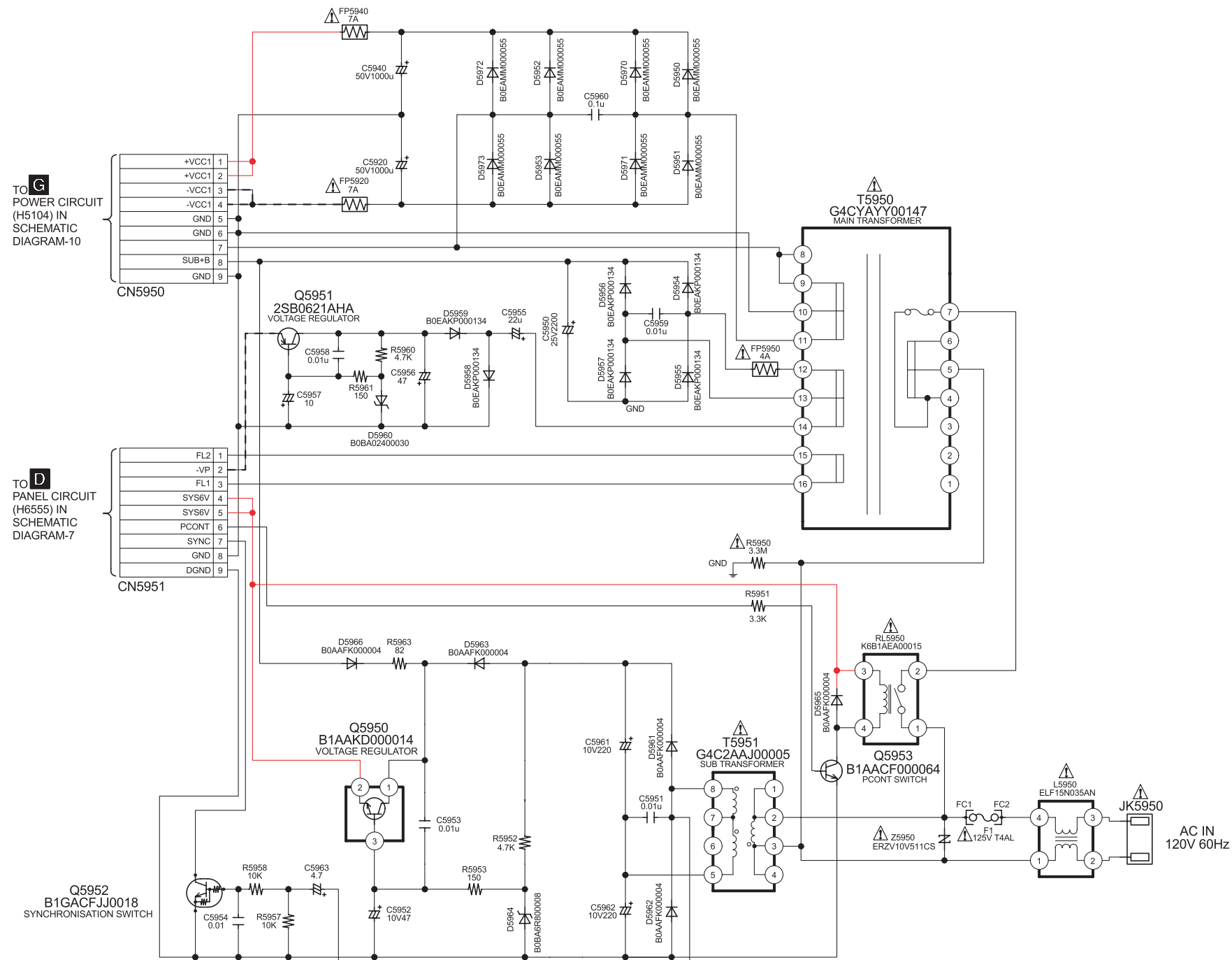
SCHEMATIC DIAGRAM - 12 J TRANSFORMER CIRCUIT
