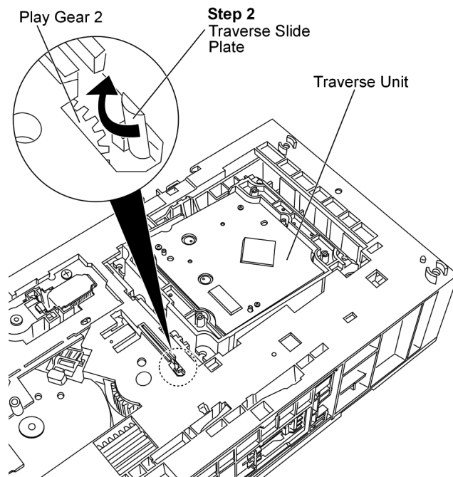
Step 2: Push the traverse slide plate as arrow shown to lock the traverse unit.
