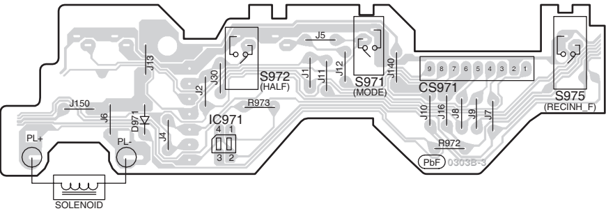
I DECK MECHANISM P.C.B (REPX0321F)
