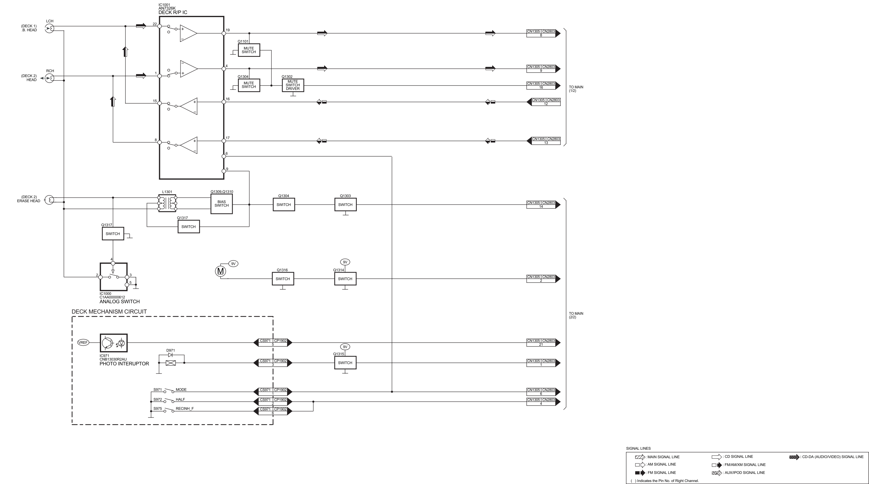
SA-AK450P/PC DECK/DECK MECHANISM BLOCK DIAGRAM
