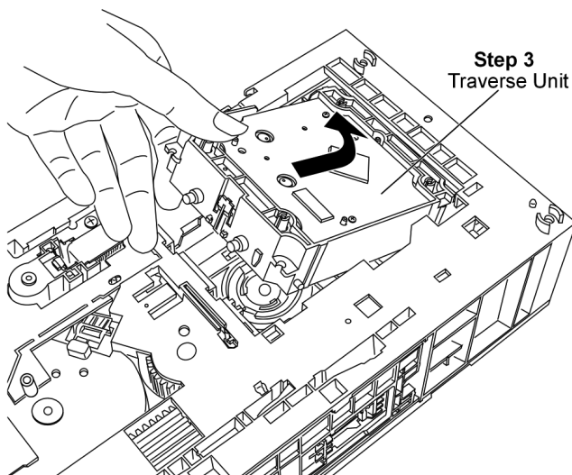
Step 3: Remove the traverse unit as arrow shown.
