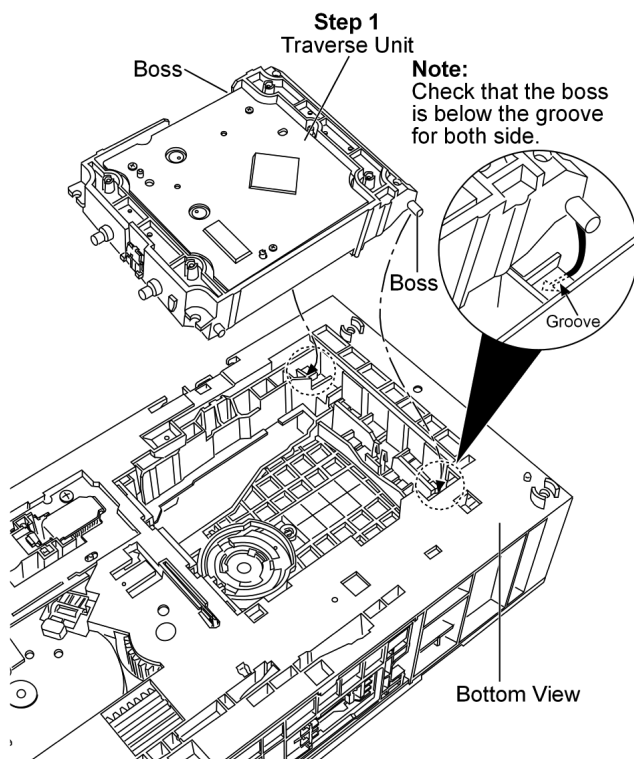
Step 1: Turn over the unit and install the traverse unit.
