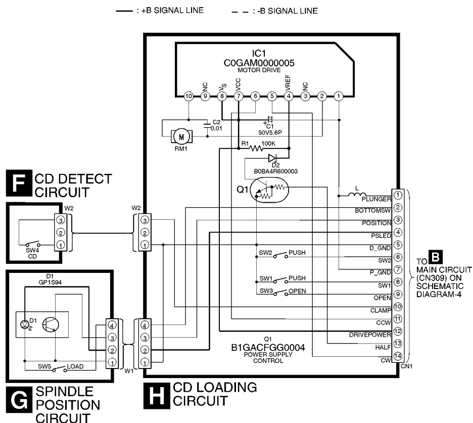
SCHEMATIC DIAGRAM - 14
