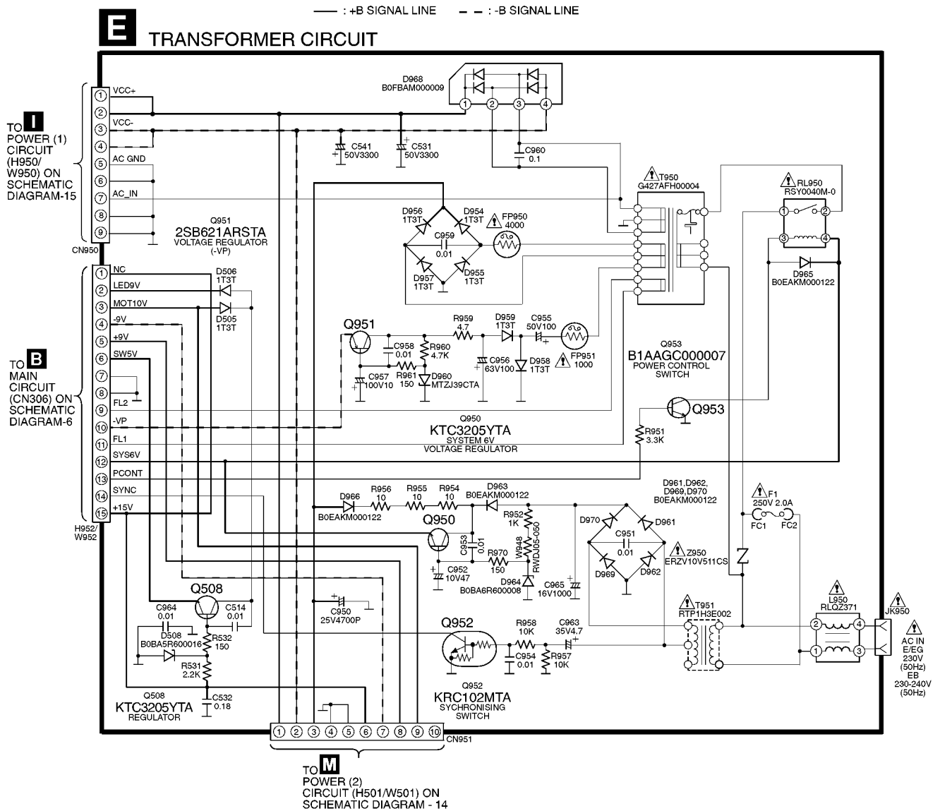
SCHEMATIC DIAGRAM - 13
