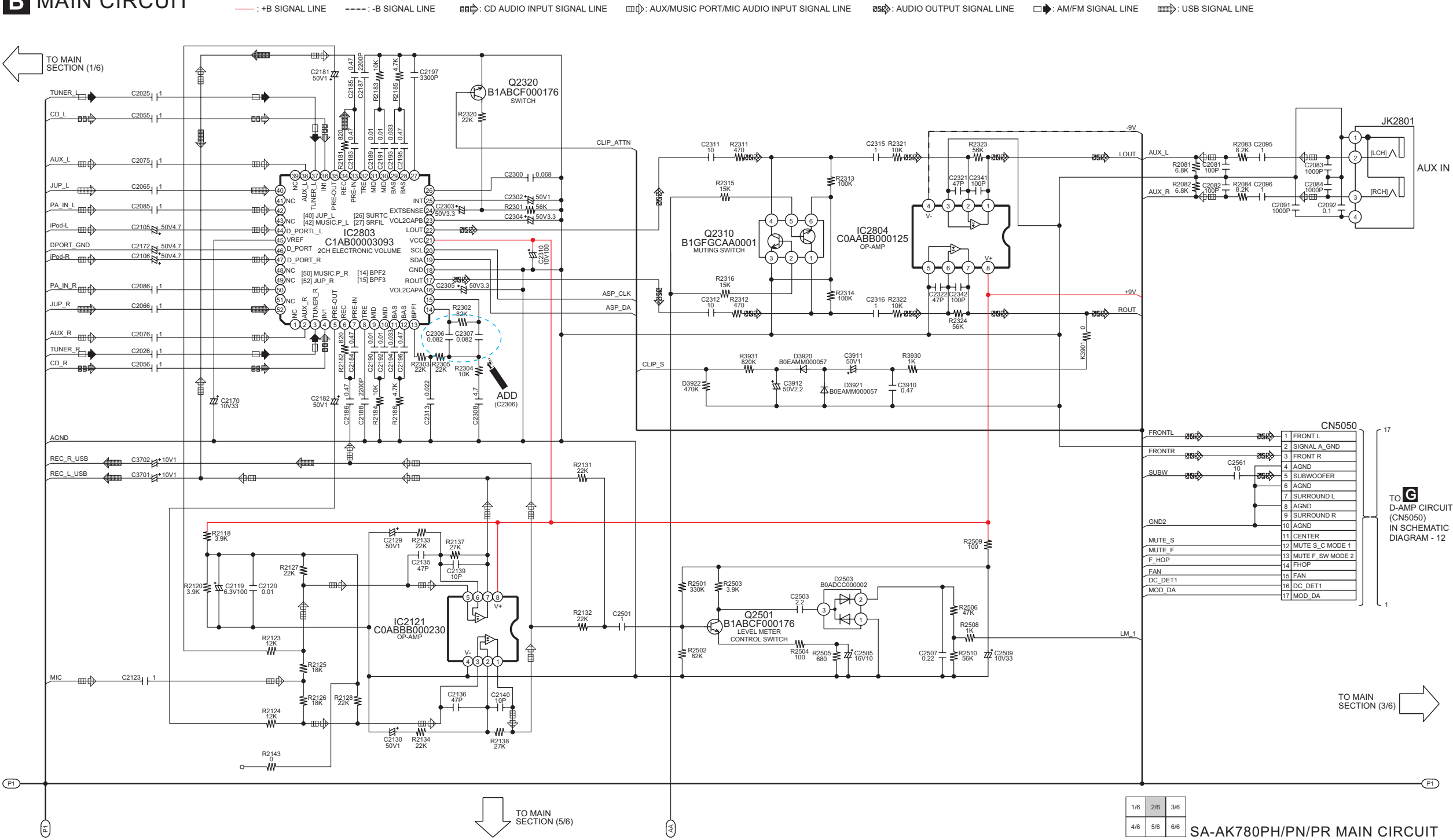
SCHEMATIC DIAGRAM - 3
