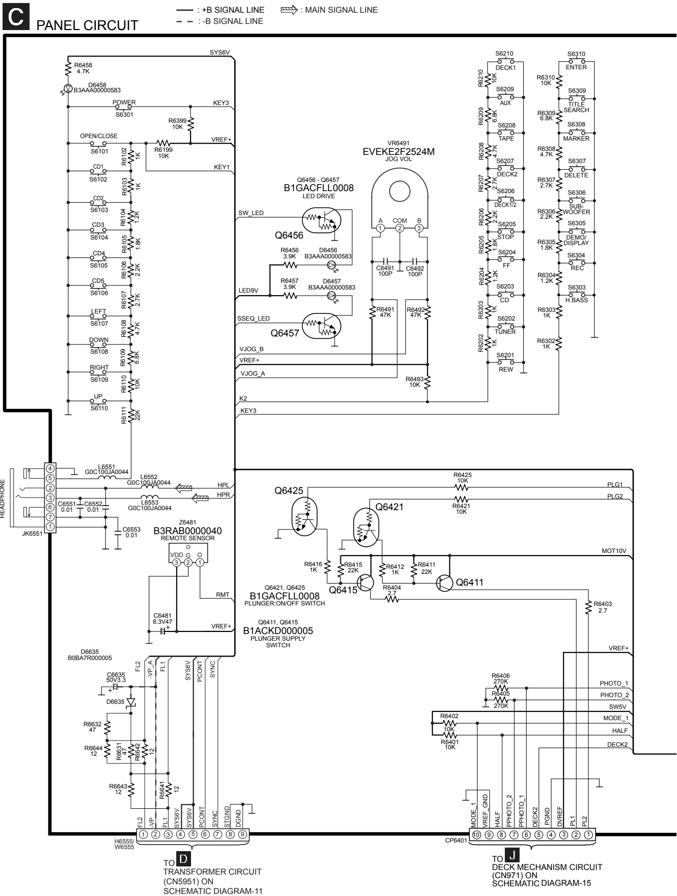
SCHEMATIC DIAGRAM - 9
