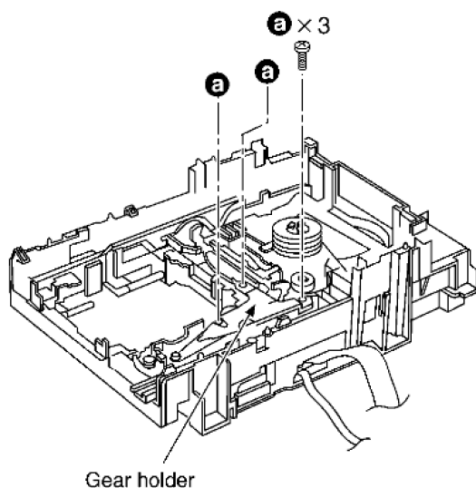
Gear holder
