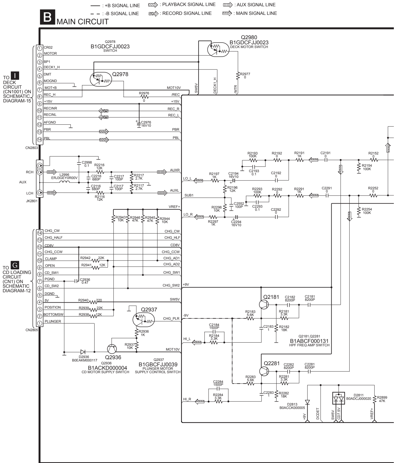
SCHEMATIC DIAGRAM - 4
