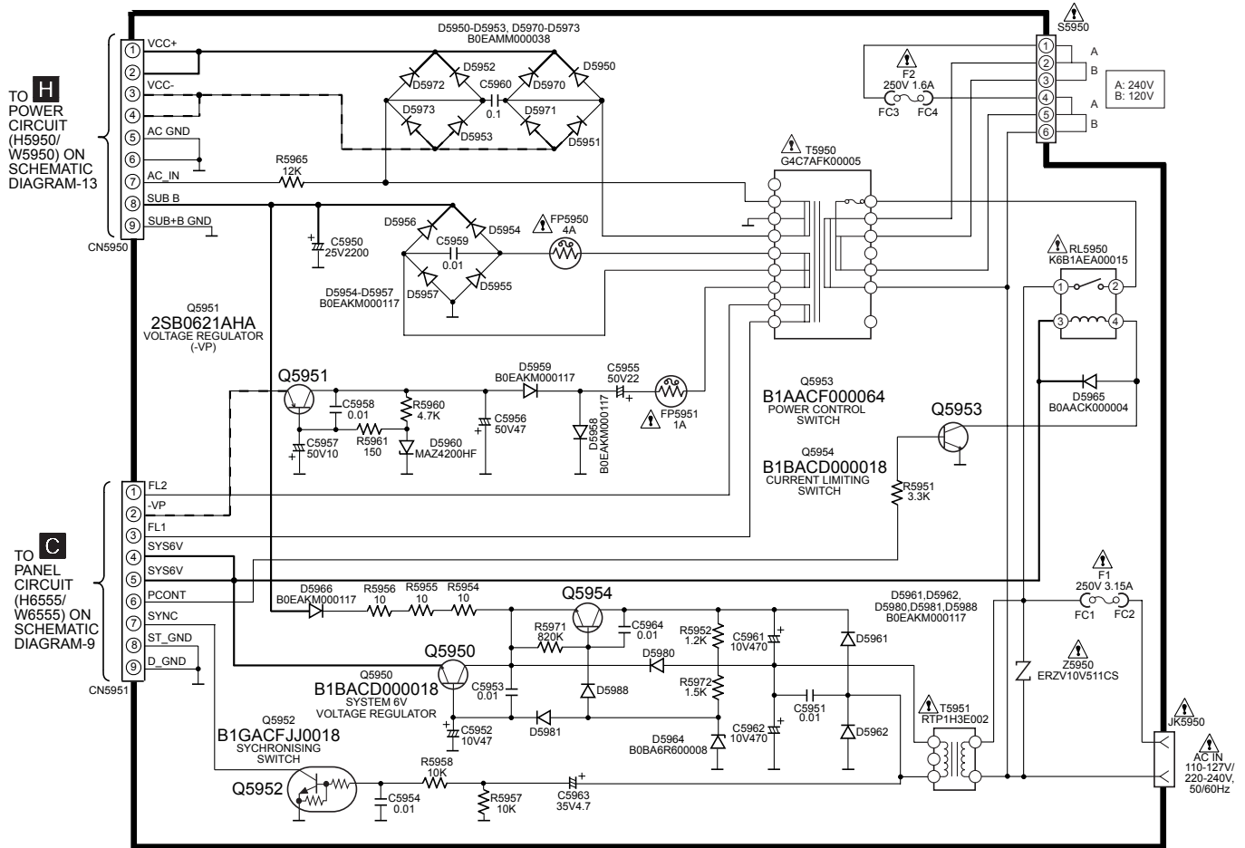
SCHEMATIC DIAGRAM - 11
