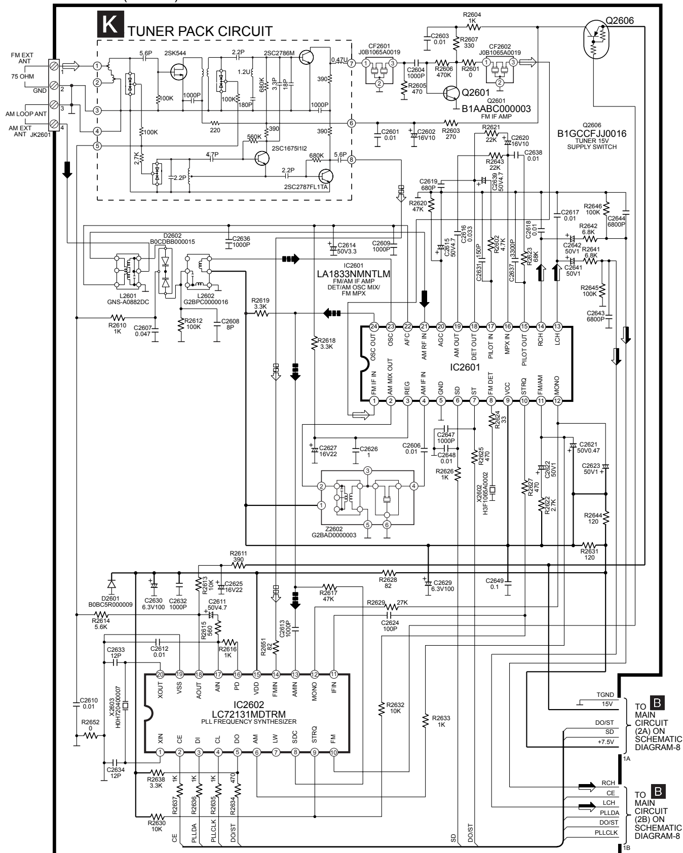
SCHEMATIC DIAGRAM - 3
