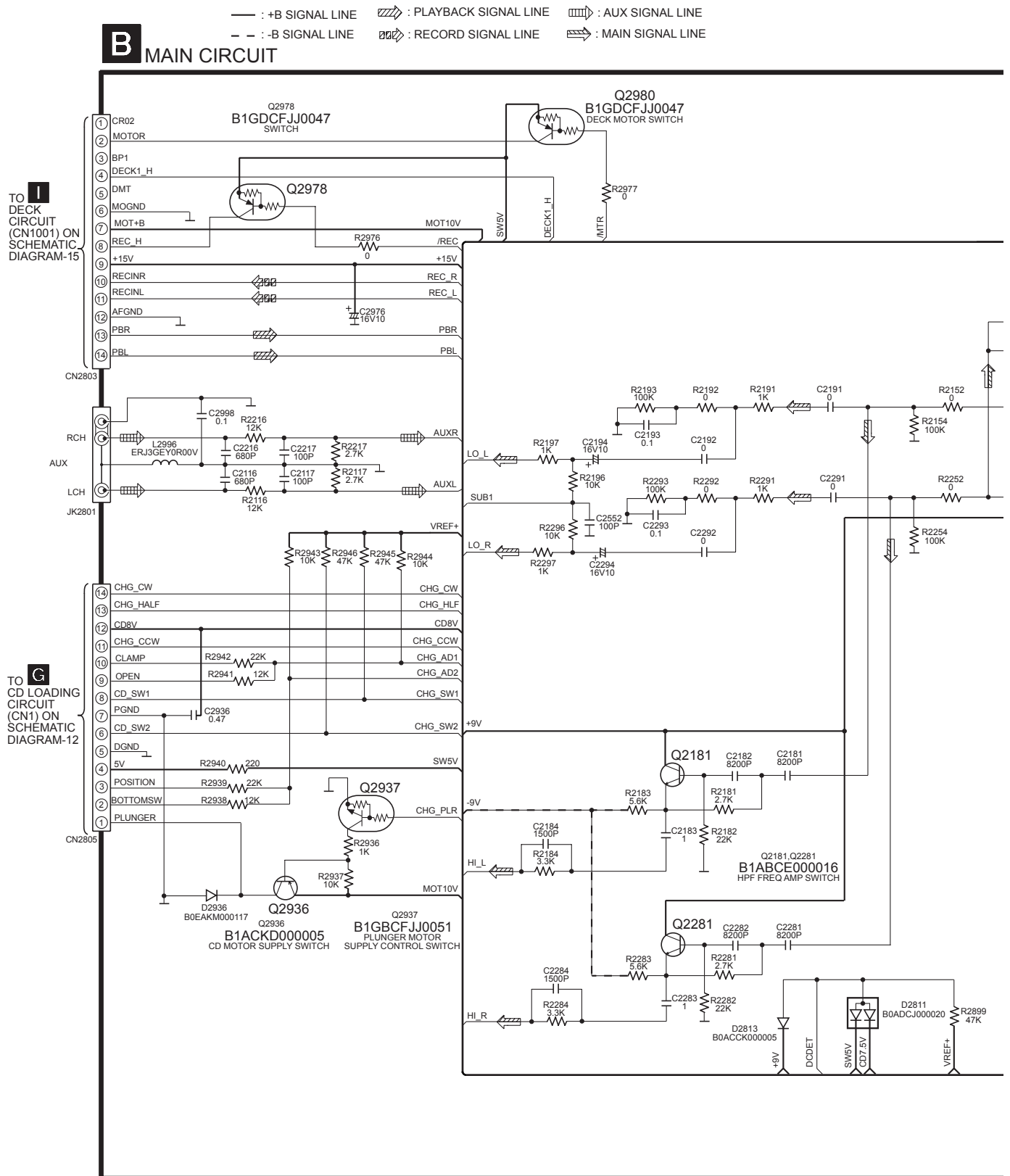
SCHEMATIC DIAGRAM - 4
