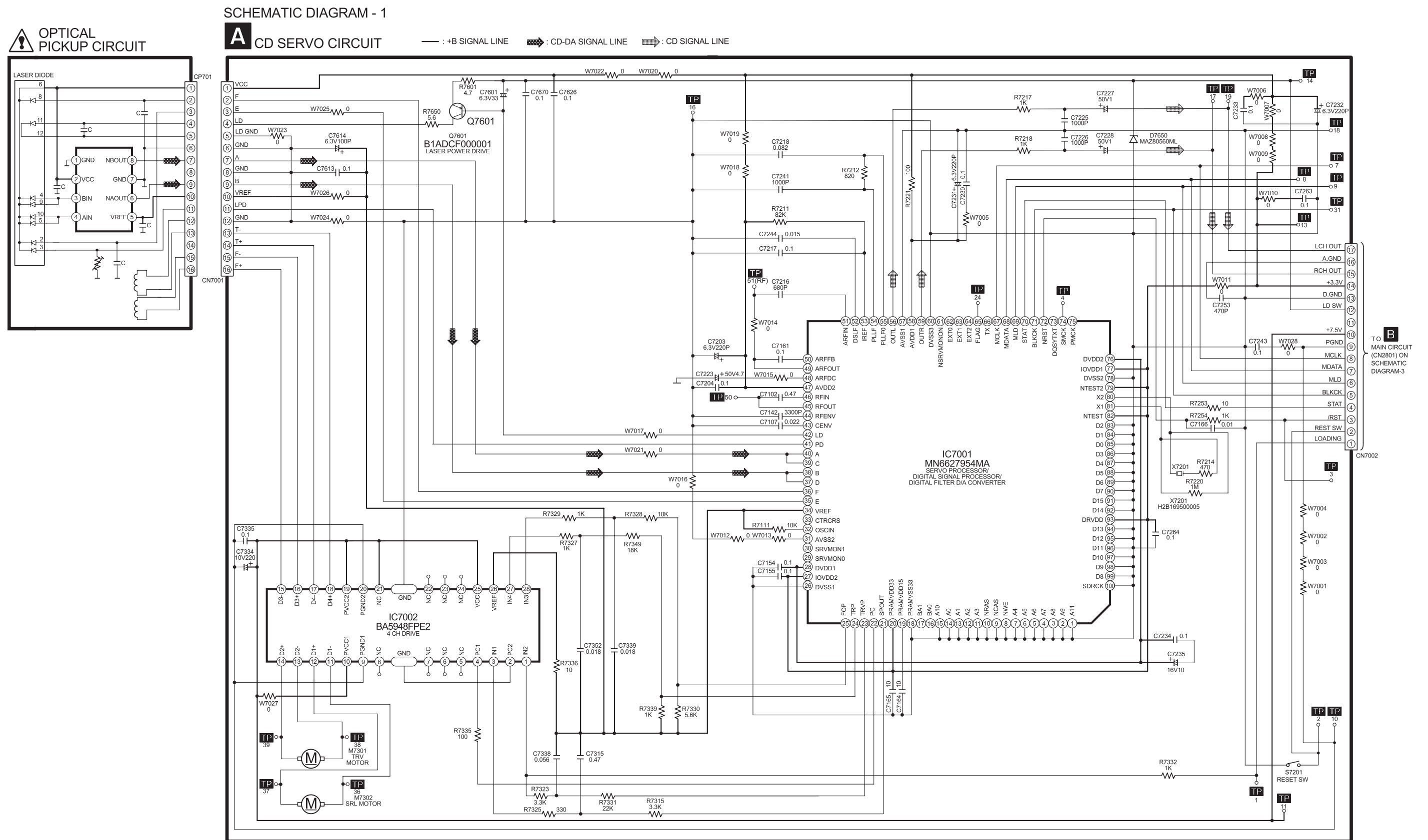
SA-AK640E/EB/EG CD SERVO CIRCUIT
