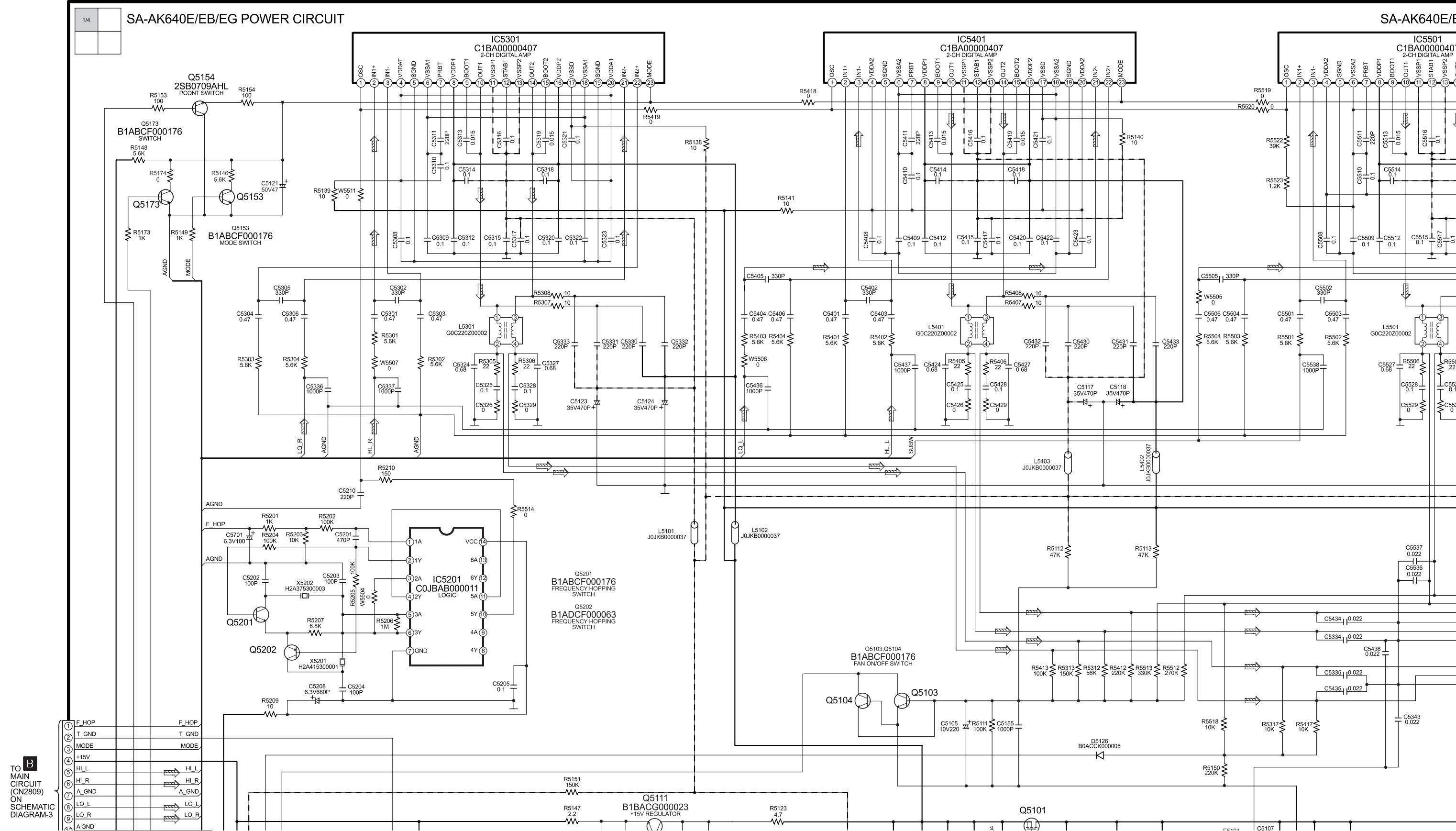
SCHEMATIC DIAGRAM - 6
