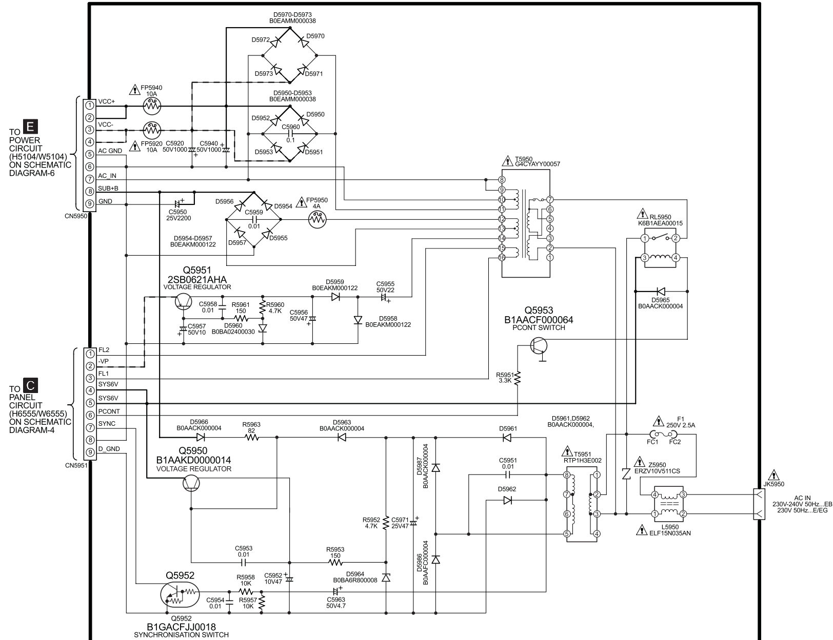
SCHEMATIC DIAGRAM - 5
