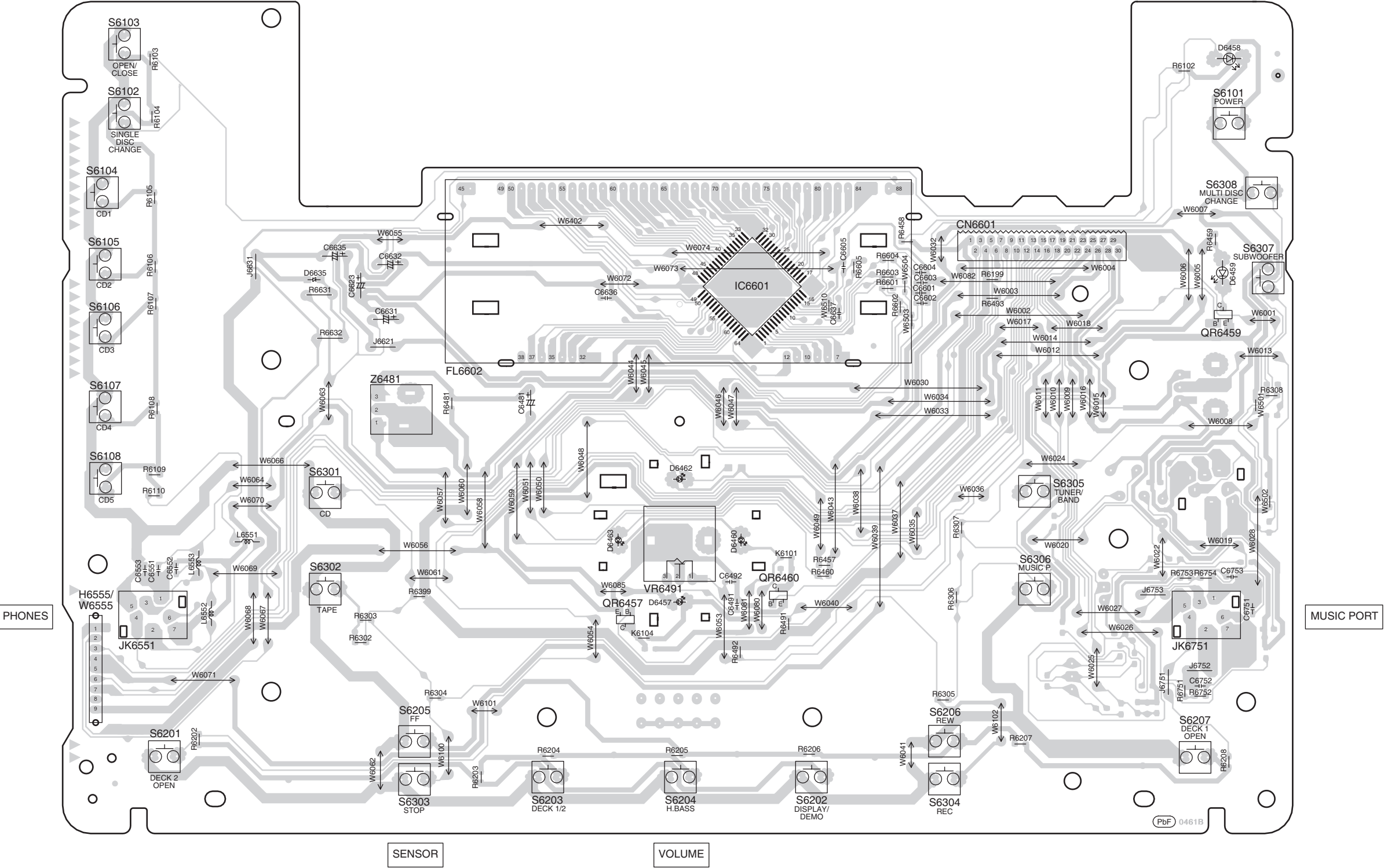
C PANEL P.C.B (REPX0517M)
