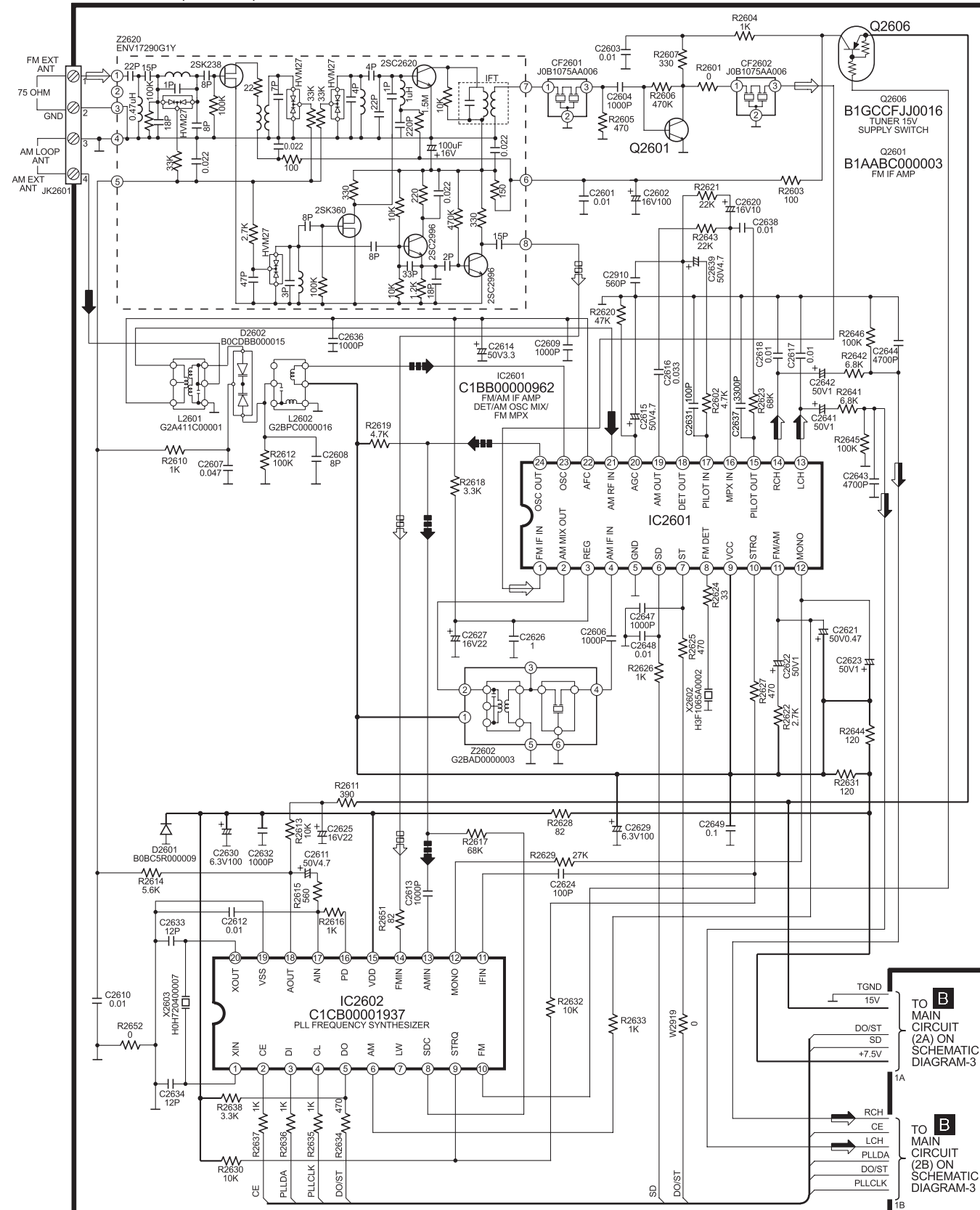
SA-AK640EE MAIN (TUNER) CIRCUIT
