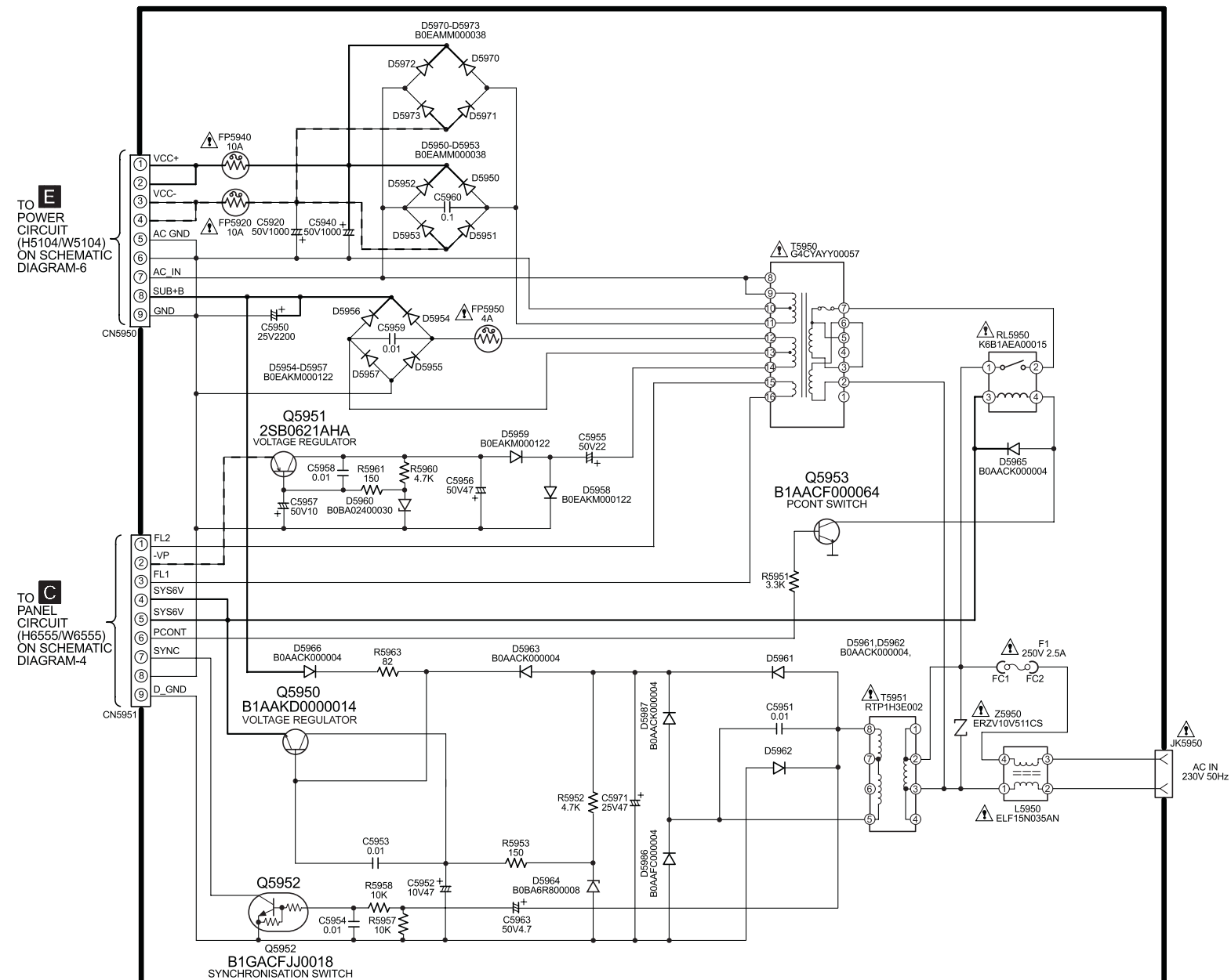
SA-AK640EE TRANSFORMER CIRCUIT
