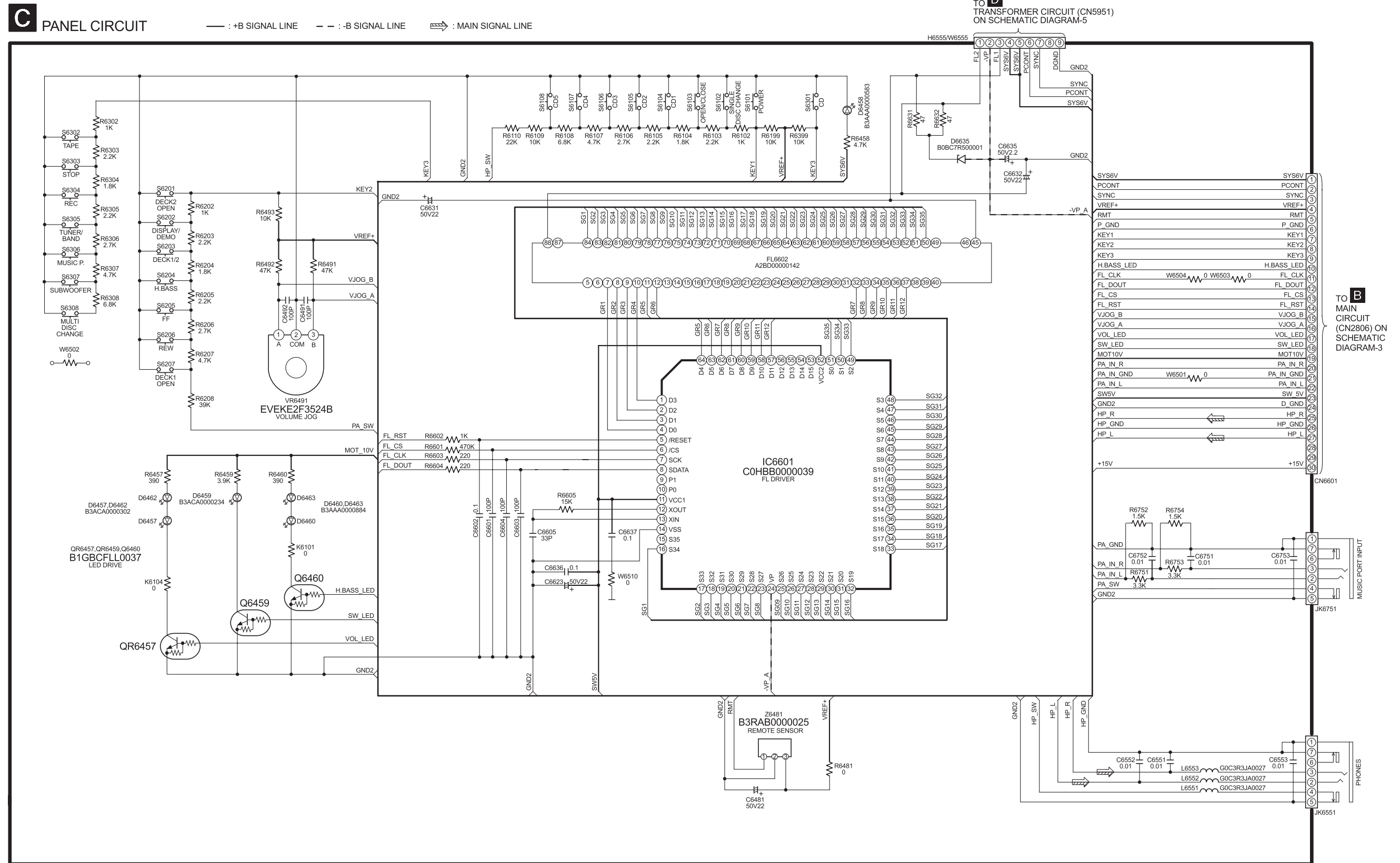
SA-AK640EE PANEL CIRCUIT
