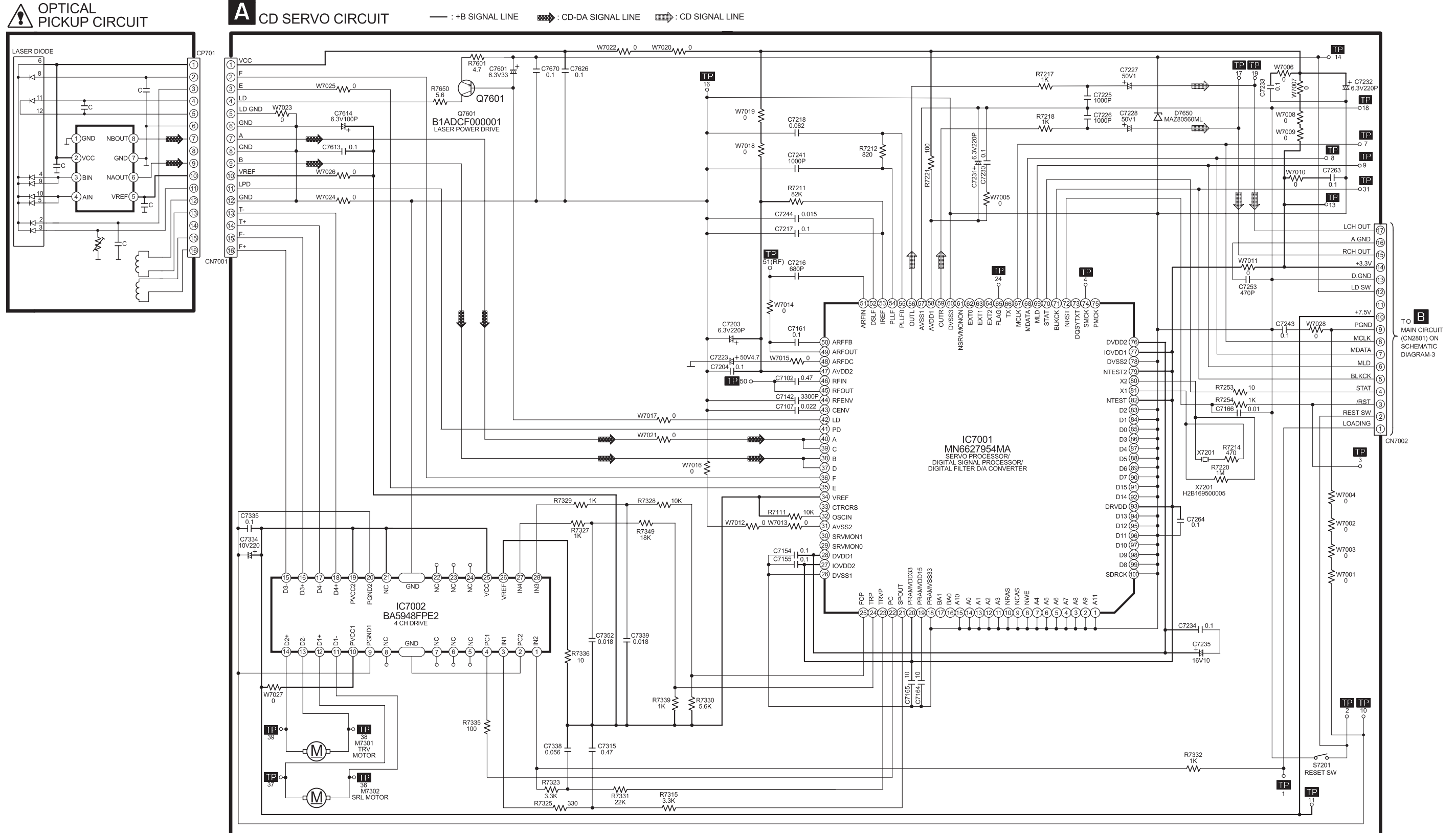
SA-AK640EE CD SERVO CIRCUIT
