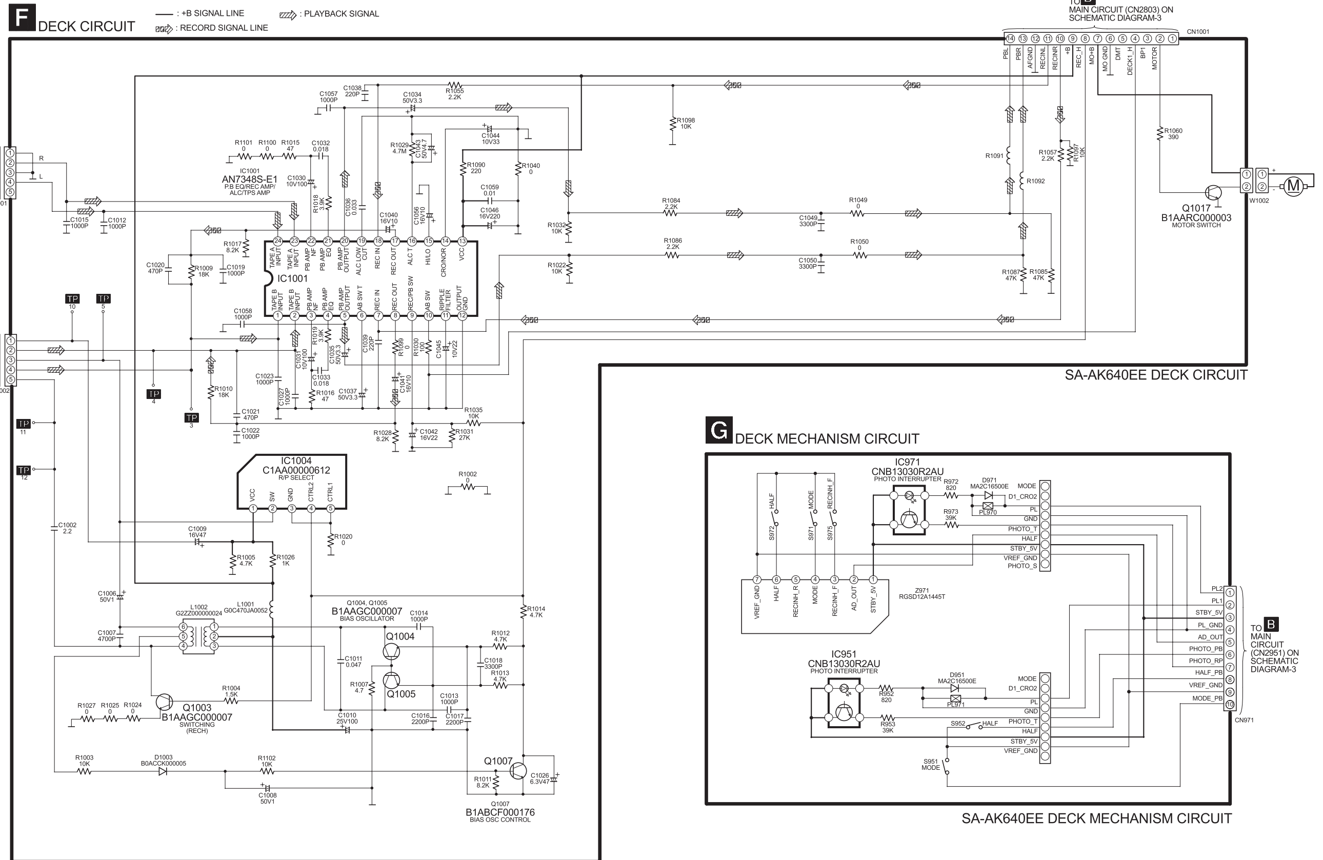
SCHEMATIC DIAGRAM - 7
