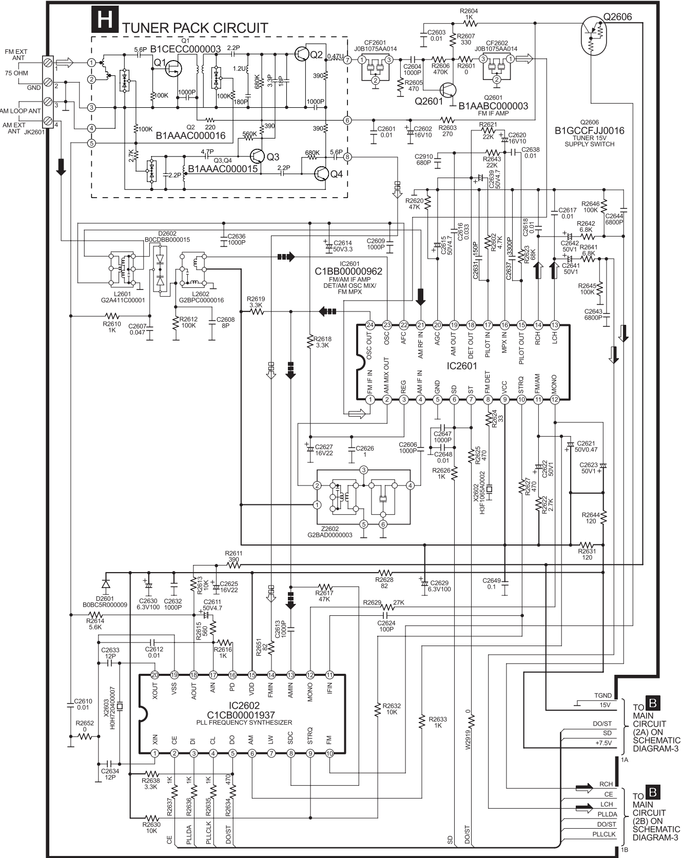
SA-AK640GCP MAIN(TUNER) CIRCUIT
