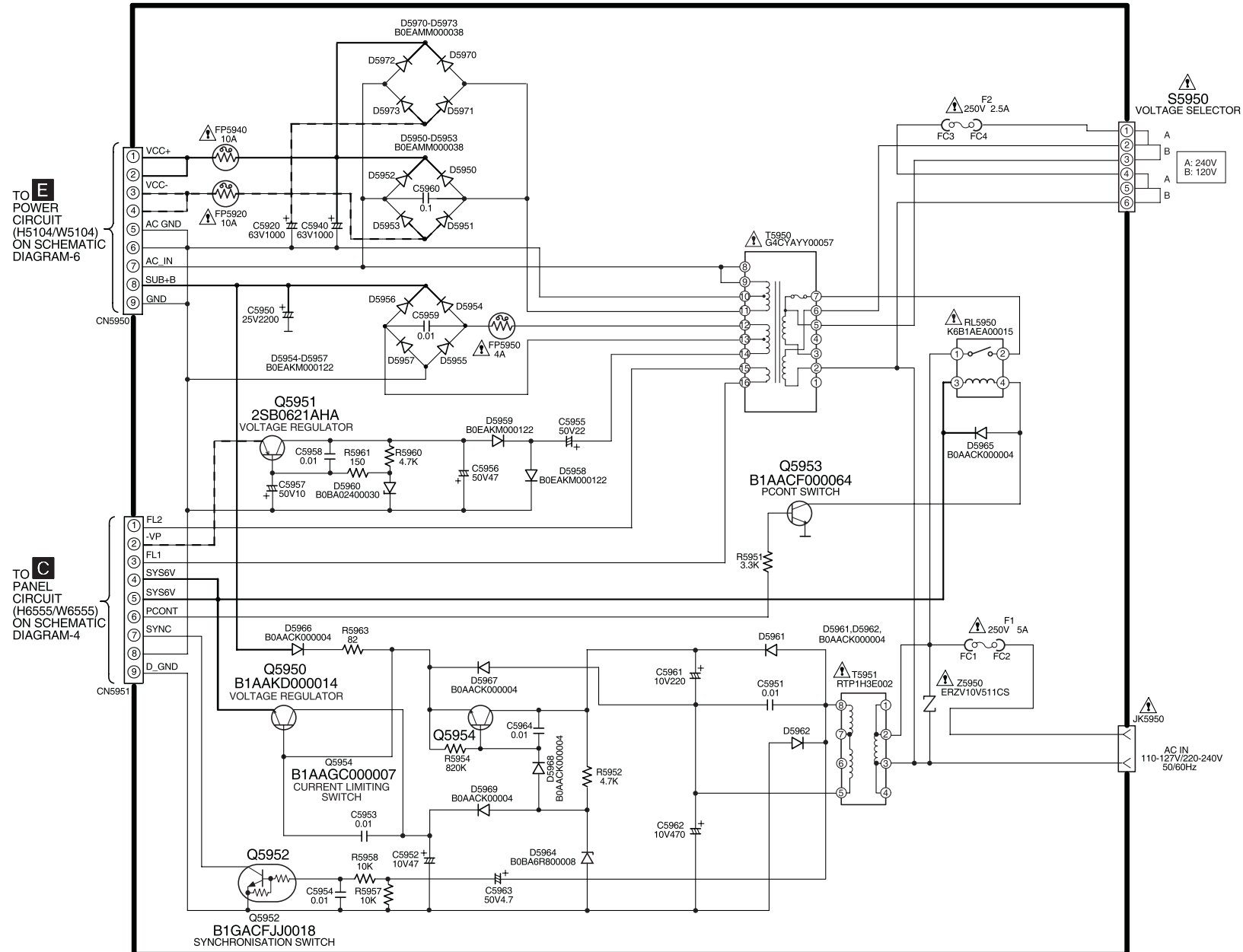
SA-AK640GCP TRANSFORMER CIRCUIT
