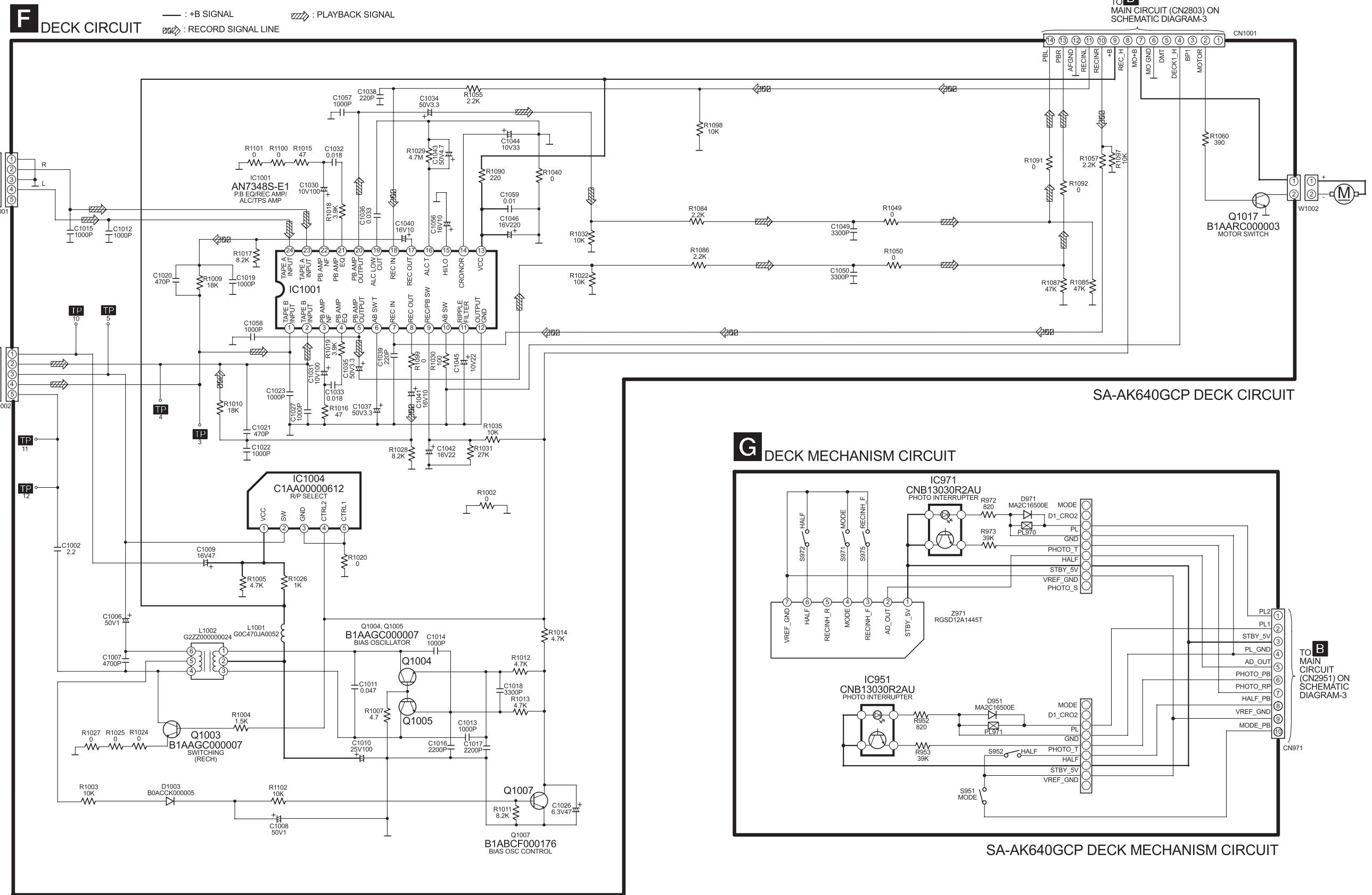
SCHEMATIC DIAGRAM - 7
