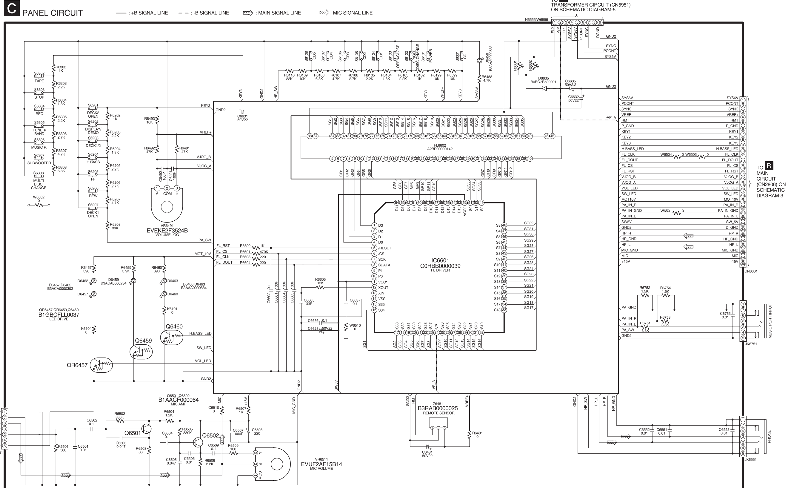
SCHEMATIC DIAGRAM - 4
